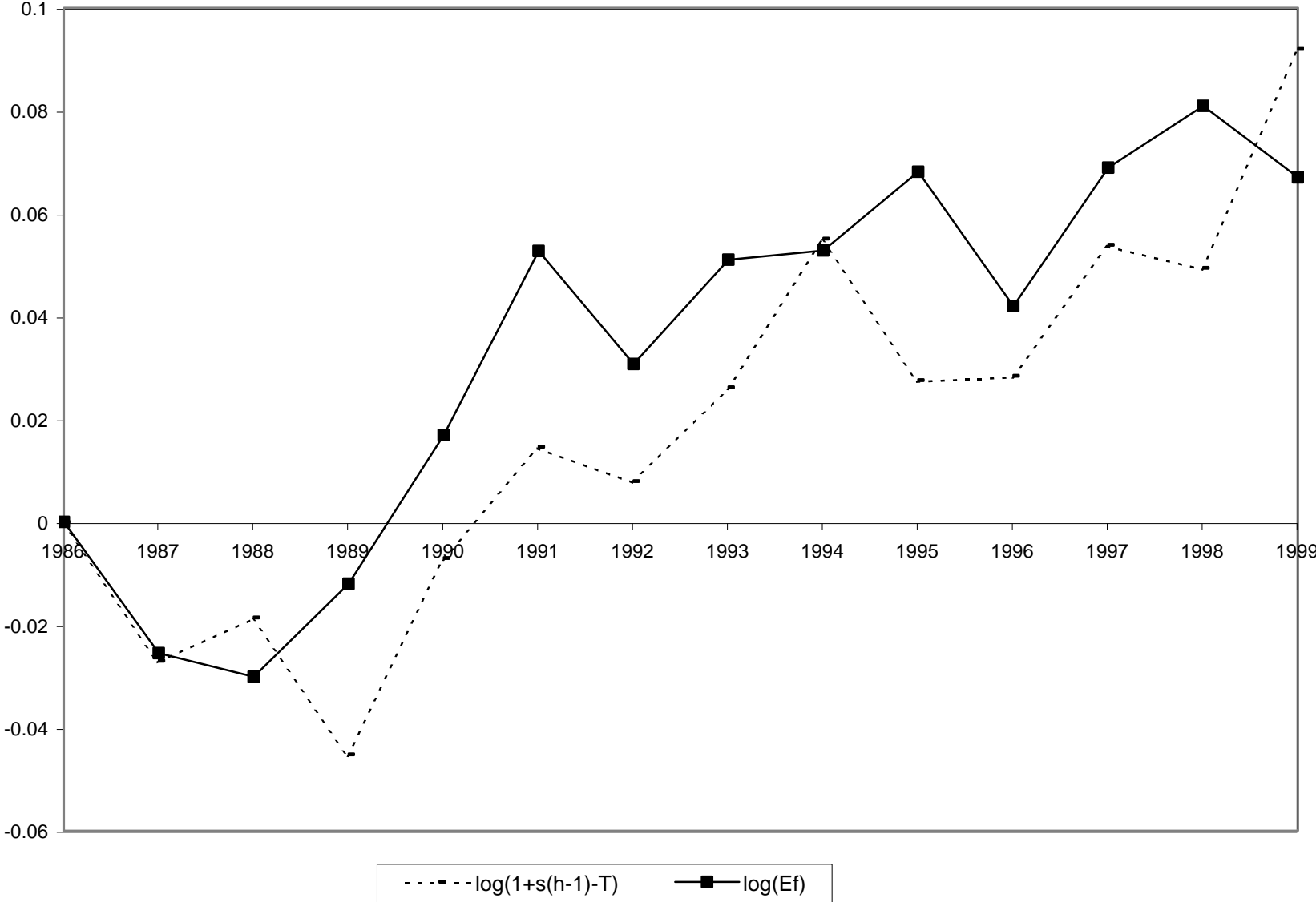
Figure 6: Coefficient of the interaction between program intensity and survey year dummies. Dependent variable: \log(E_f) and \log(1+s(h-1)-T)
