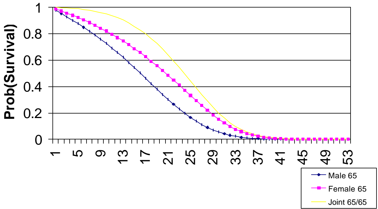
Figure 1: Individual and Joint Survival
