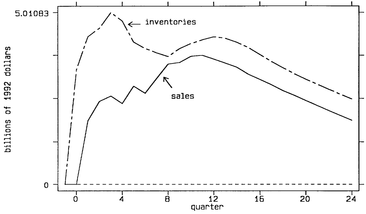
Figure 4: Response to Inventory Equation Shock, Quarterly VAR
