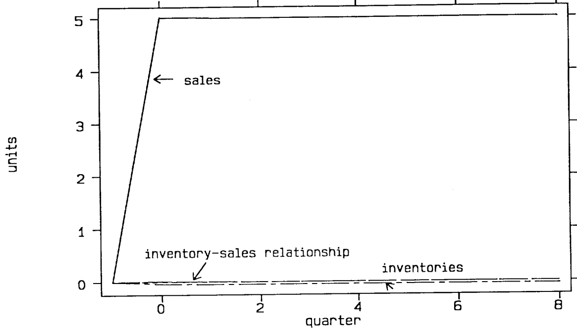
Figure 10: Response to a Unit Root Demand Shock Parameter Set A'
