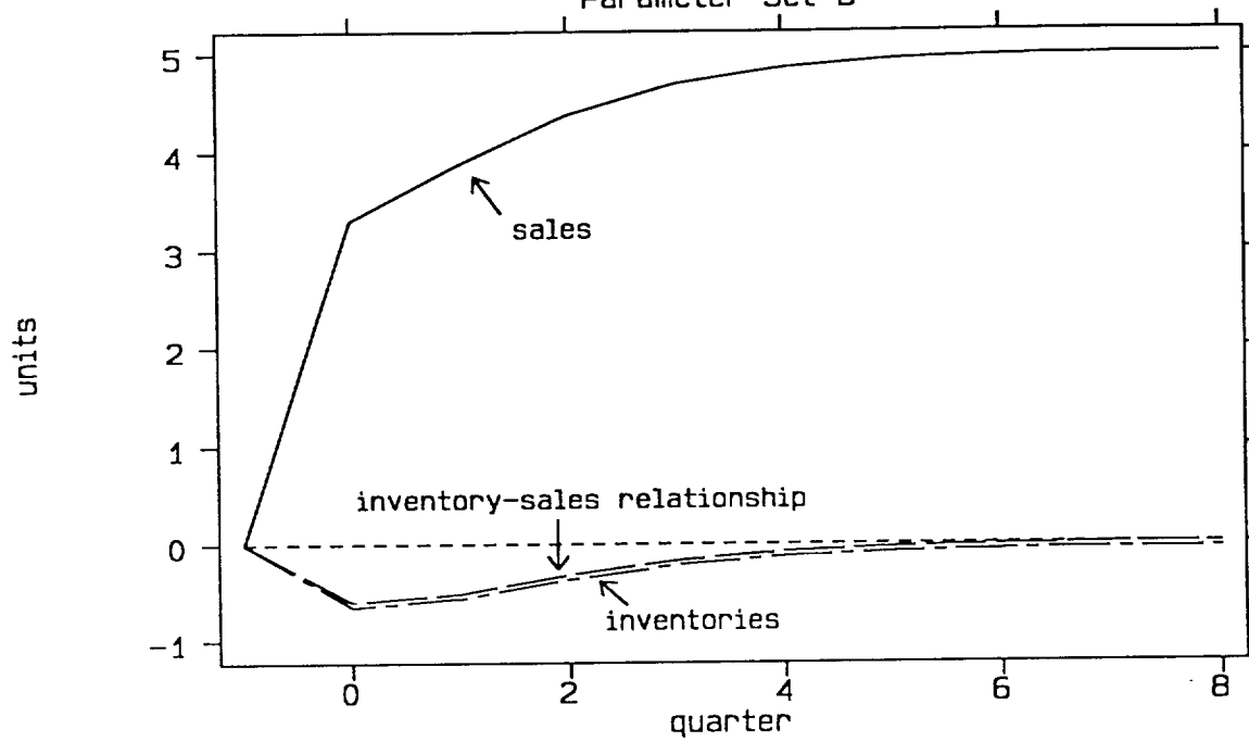
Figure 12: Response to a Unit Root Demand Shock Parameter Set D
