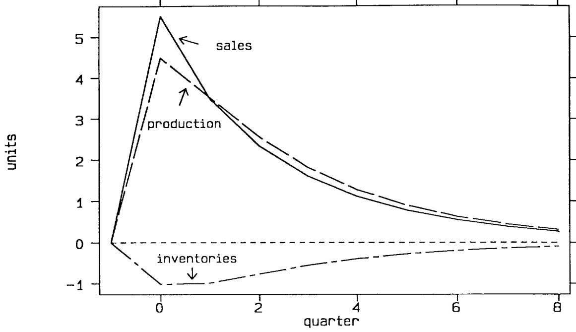
Figure 7: Response to a Stationary Demand Shock Parameter Set A
