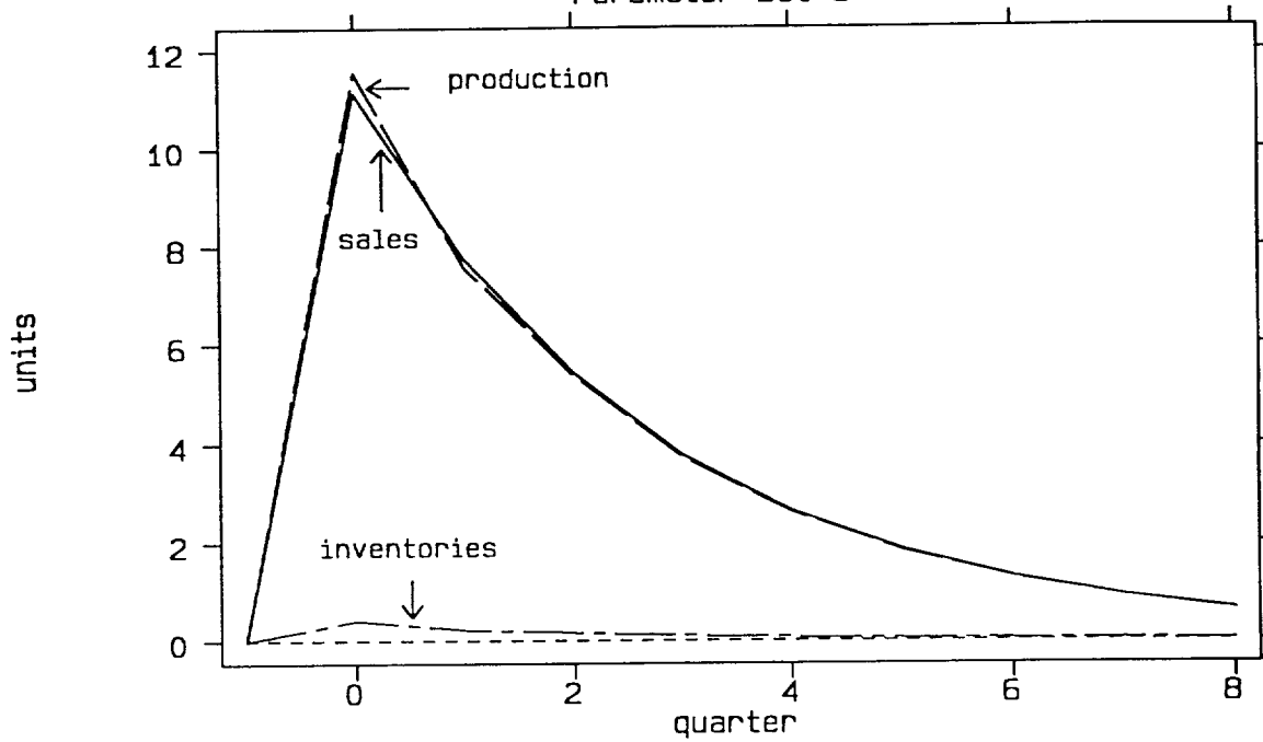
Figure 9: Response to a Stationary Demand Shock Parameter Set C
