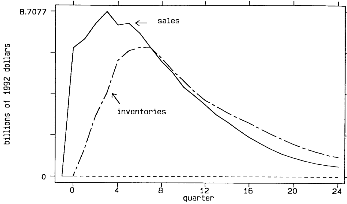
Figure 3: Response to Sales Equation Shock, Quarterly VAR
