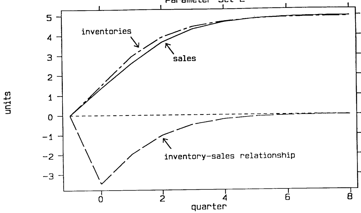
Figure 13: Response to a Unit Root Demand Shock Parameter Set E
