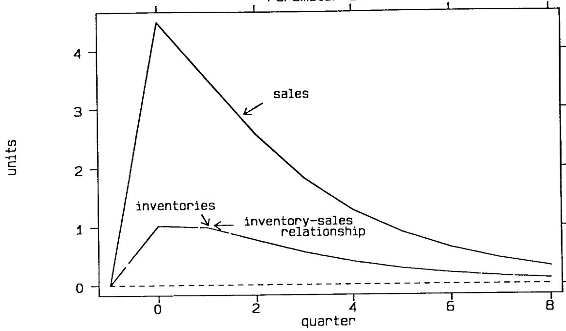
Figure 11: Response to a Stationary Cost Shock Parameter Set A''
