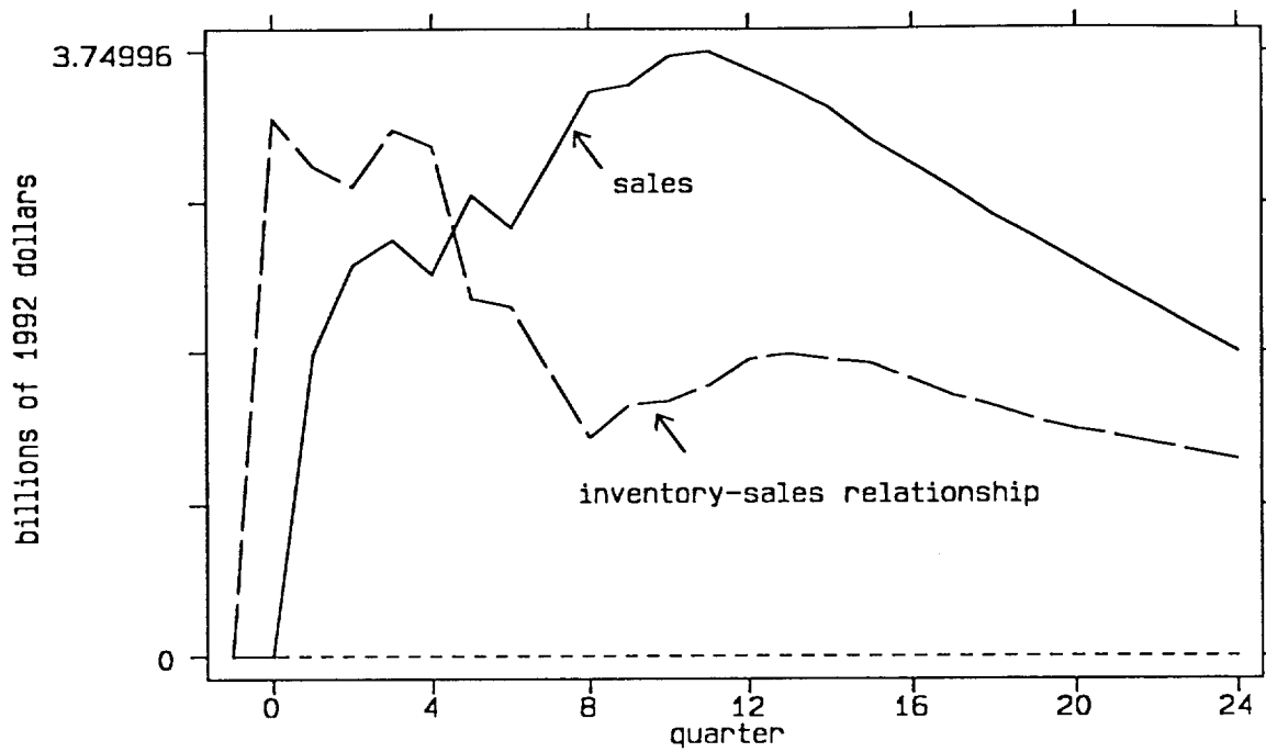
Figure 6: Response to Inventory Equation Shock, Quarterly VAR
