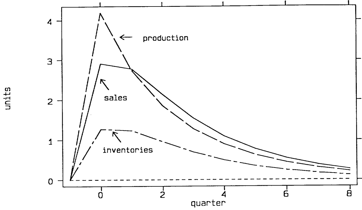
Figure 8: Response to a Stationary Demand Shock Parameter Set B
