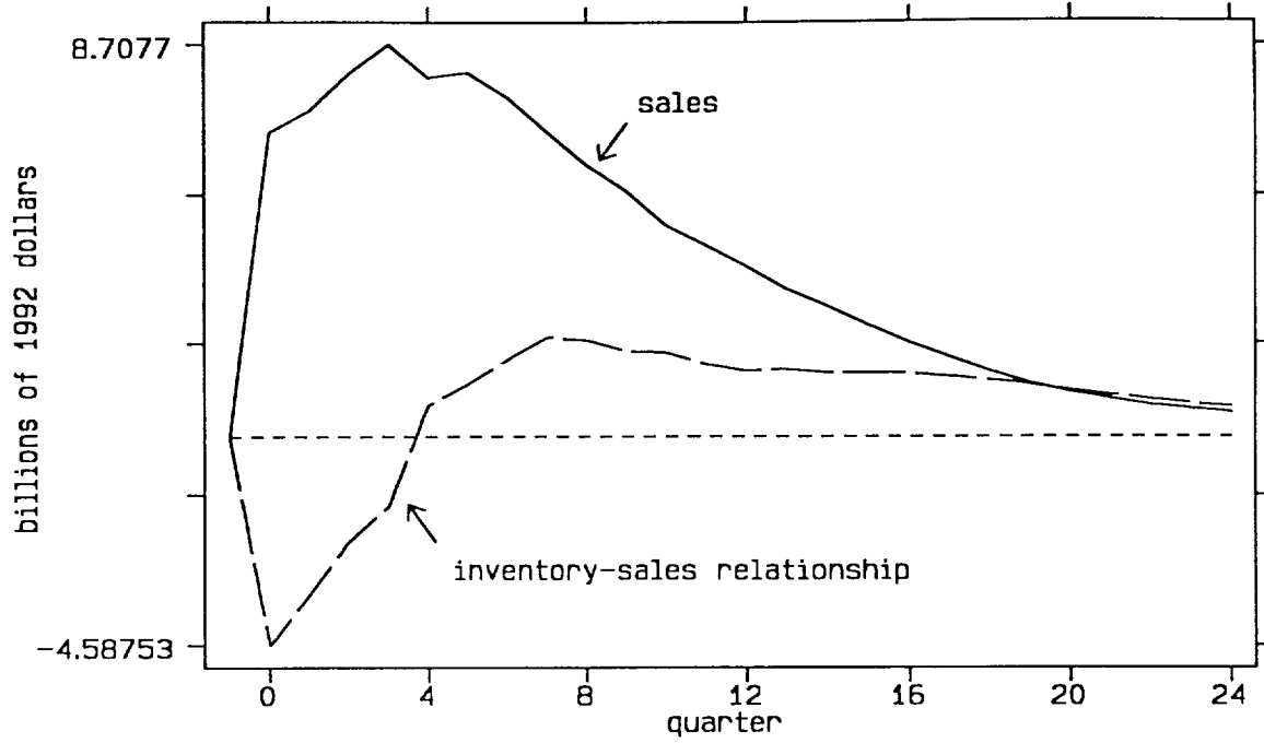
Figure 5: Response to Sales Equation Shock, Quarterly VAR
