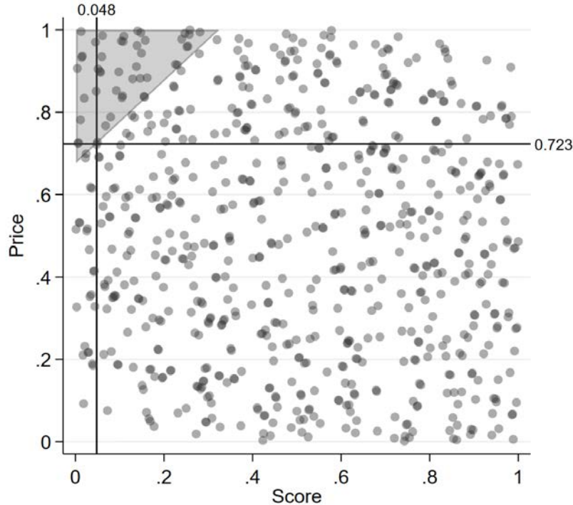
Figure 7: Scatter plot of the quantiles of the two tests.
