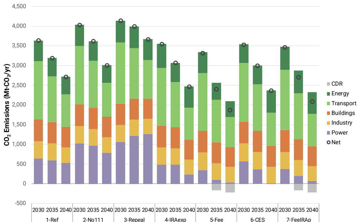
Figure 5: Projected sectoral CO 2 emissions over time by scenario. CDR = carbon dioxide removal.
