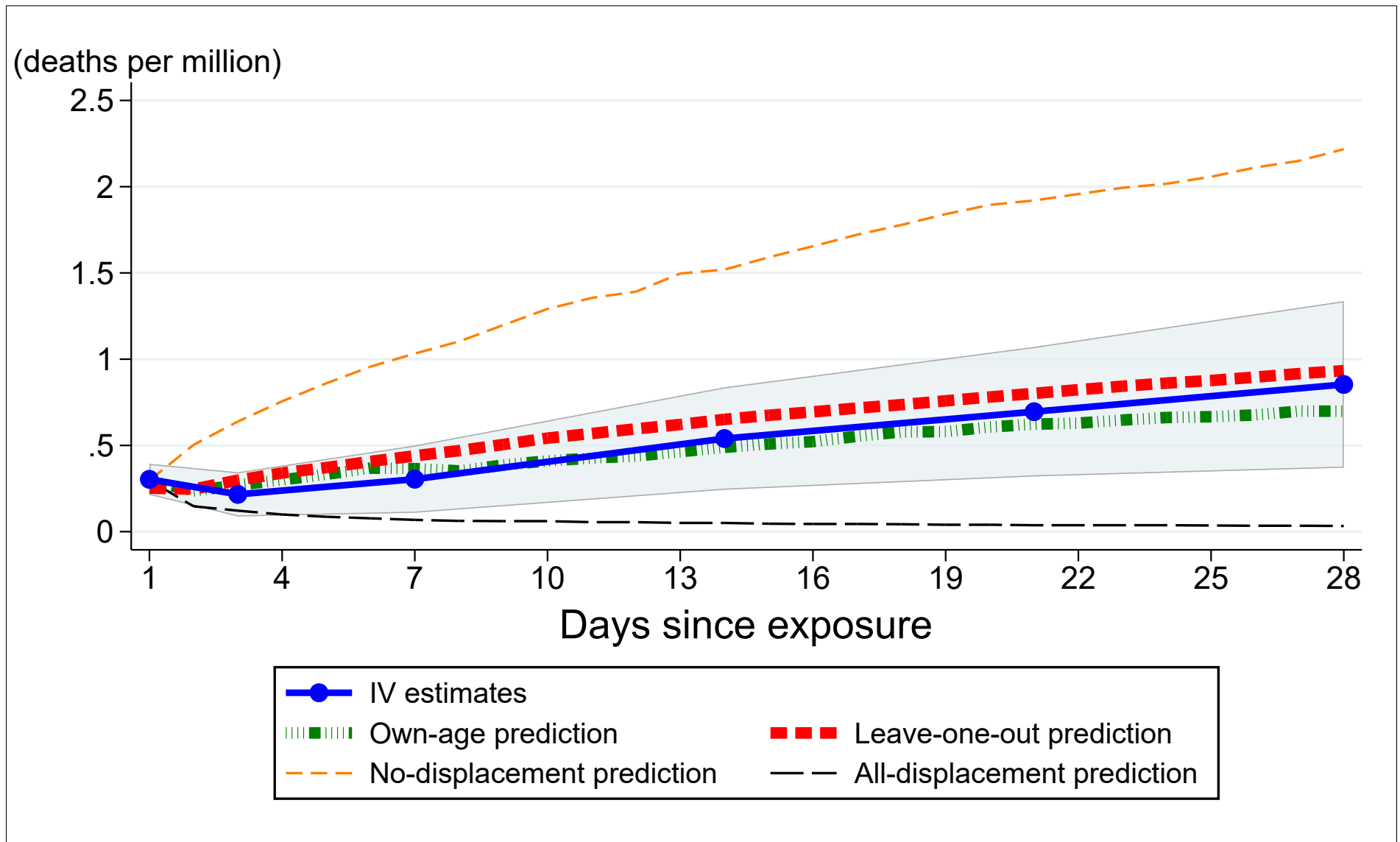
Figure V: Model predictions of effect of acute (1-day) SO 2 exposure on one-month survival, ages 65–69
