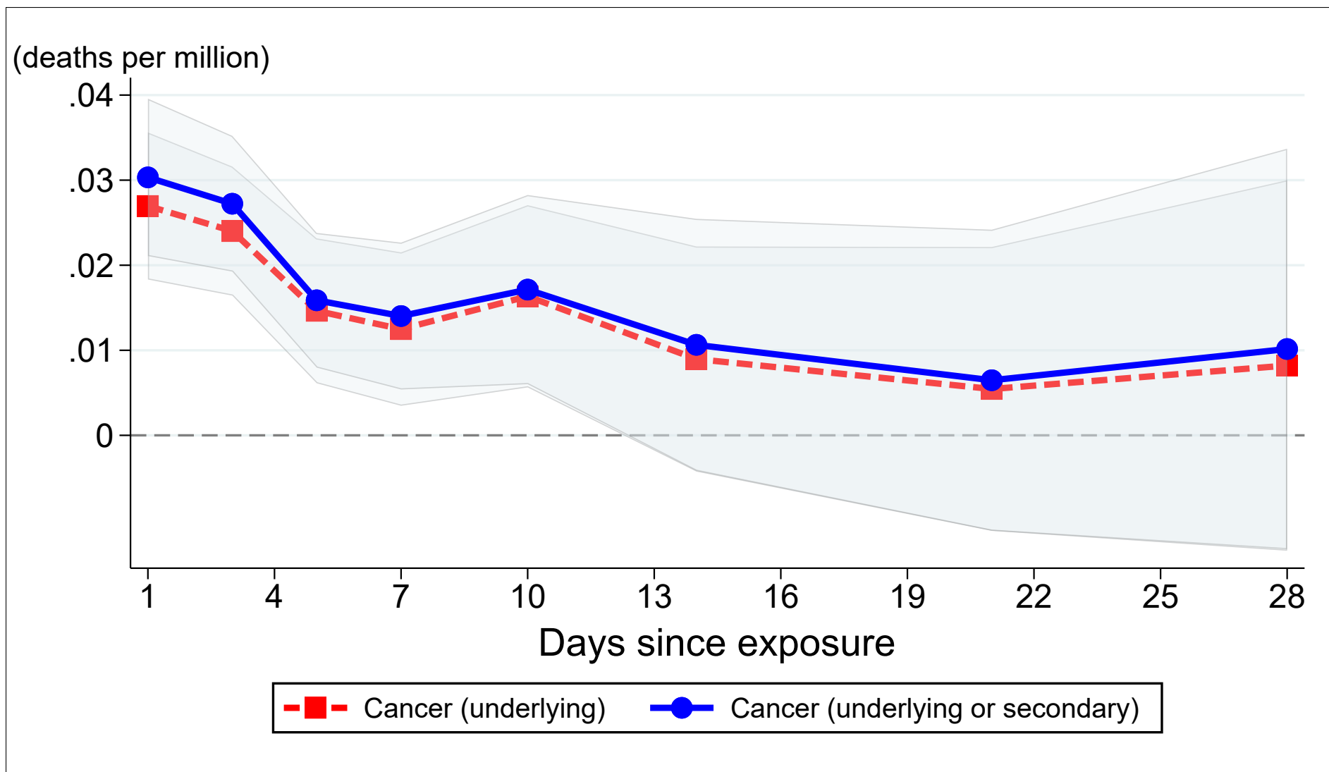
Figure A.9: IV estimates of effect of acute (1-day) SO 2 exposure on cancer-related mortality
