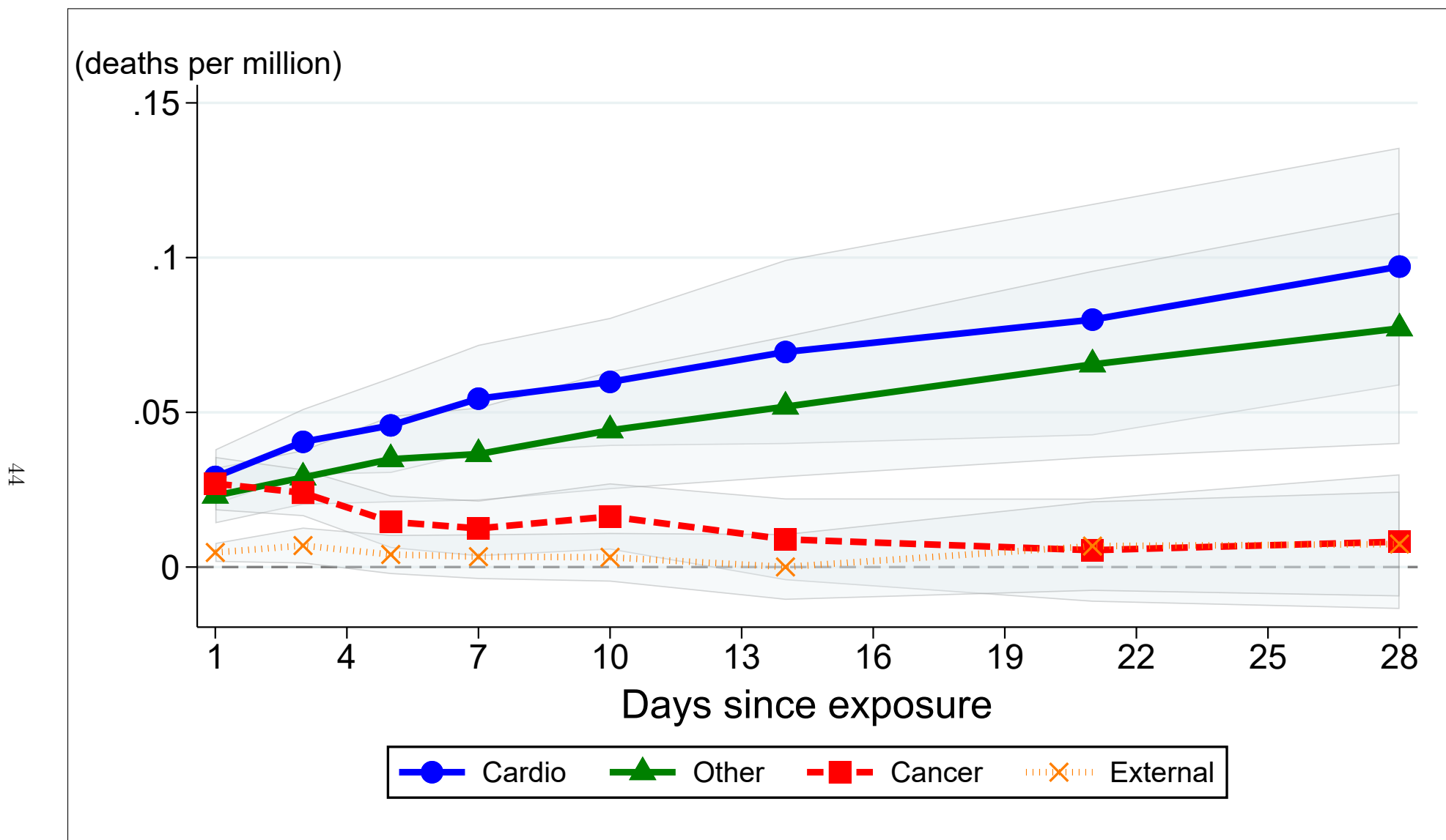
Figure III: IV estimates of effect of acute (1-day) SO 2 exposure on cumulative mortality, by cause of death
