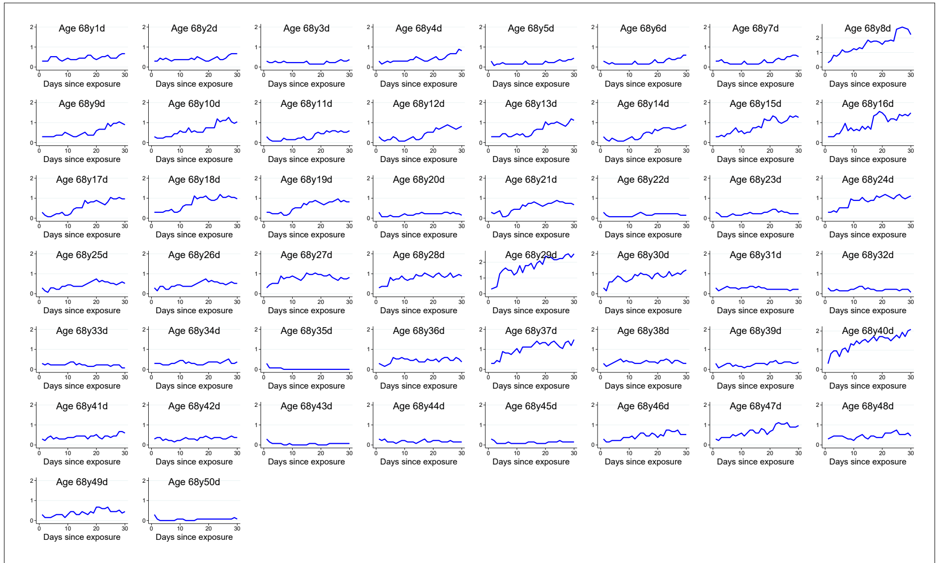
Figure A.13: Predicted effects of acute (1-day) SO 2 exposure on cumulative mortality, for selected ages
