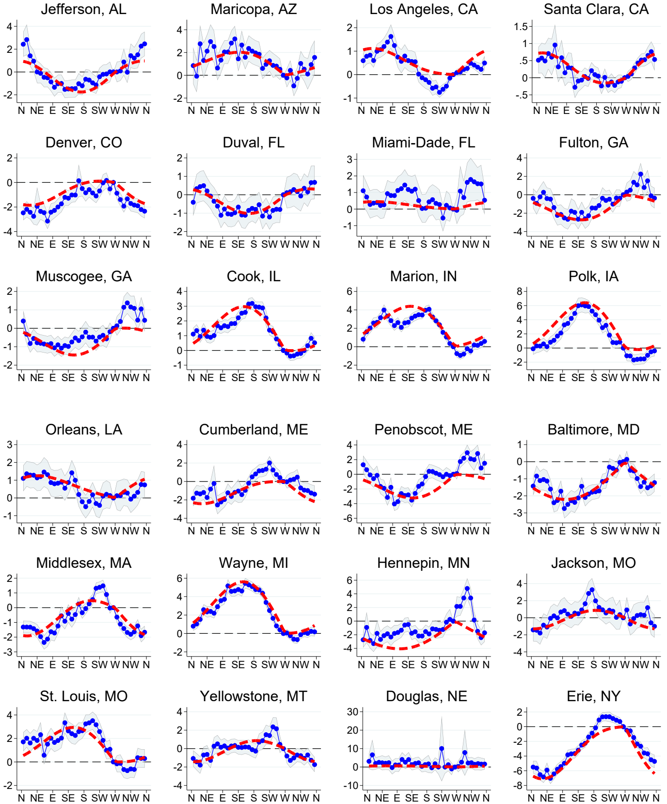
Figure A.5: The relationship between wind direction and SO 2 concentrations, by geographic group
