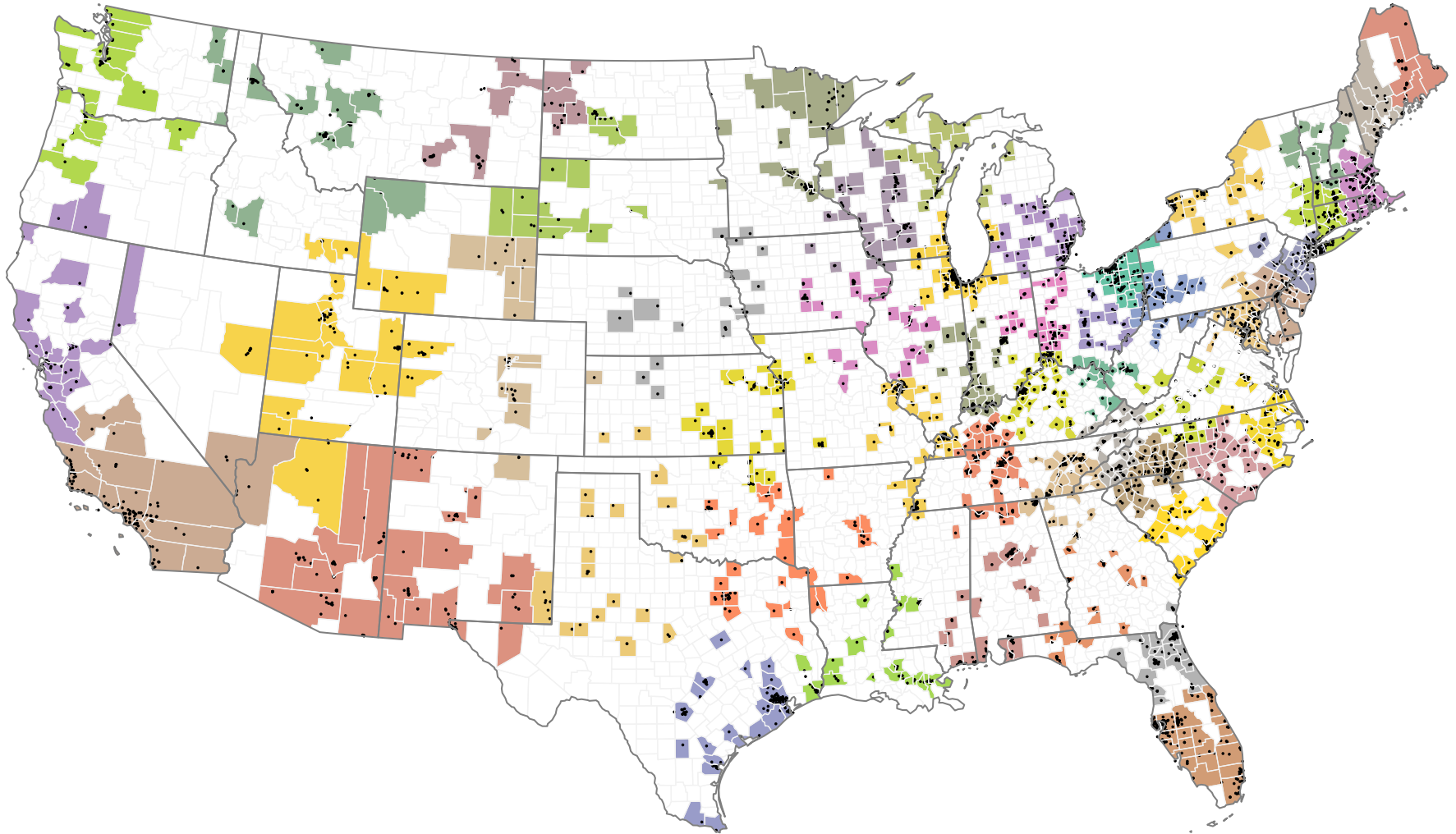
Figure A.4: Locations of the 50 geographic groups and SO 2 monitors
