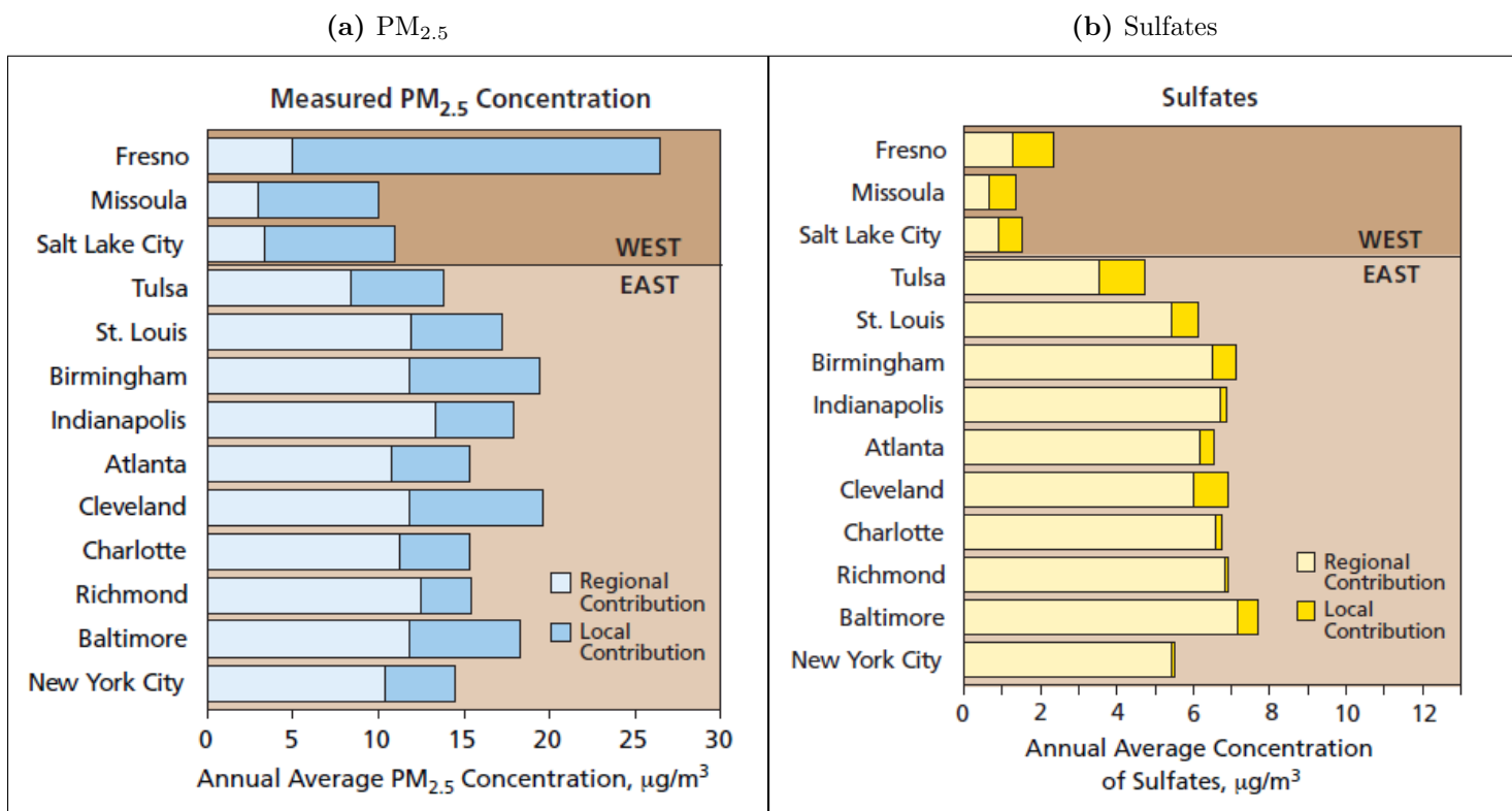
Figure A.3: Fraction of air pollution coming from non-local sources, for selected cities
