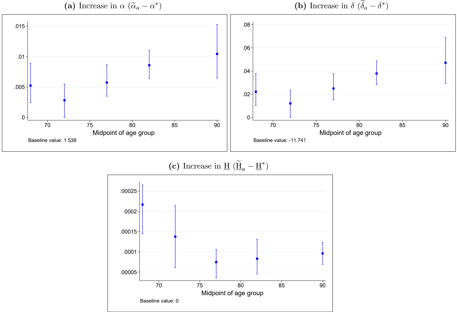
Figure A.11: The effect of acute (1-day) SO 2 exposure on model parameters
