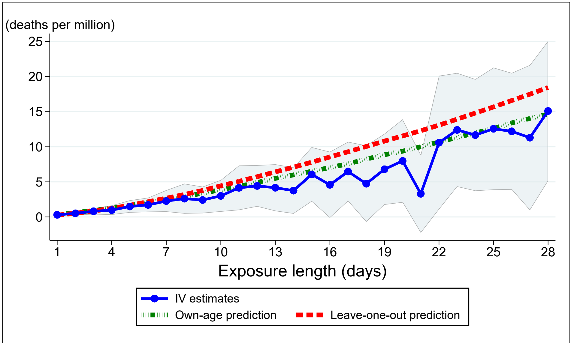
Figure VI: Model predictions of effect of short-term chronic SO 2 exposure on survival, ages 65–69
