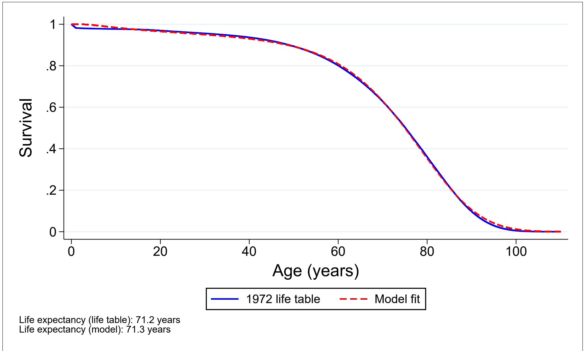
Figure A.10: Baseline calibration of the dynamic production model of health
