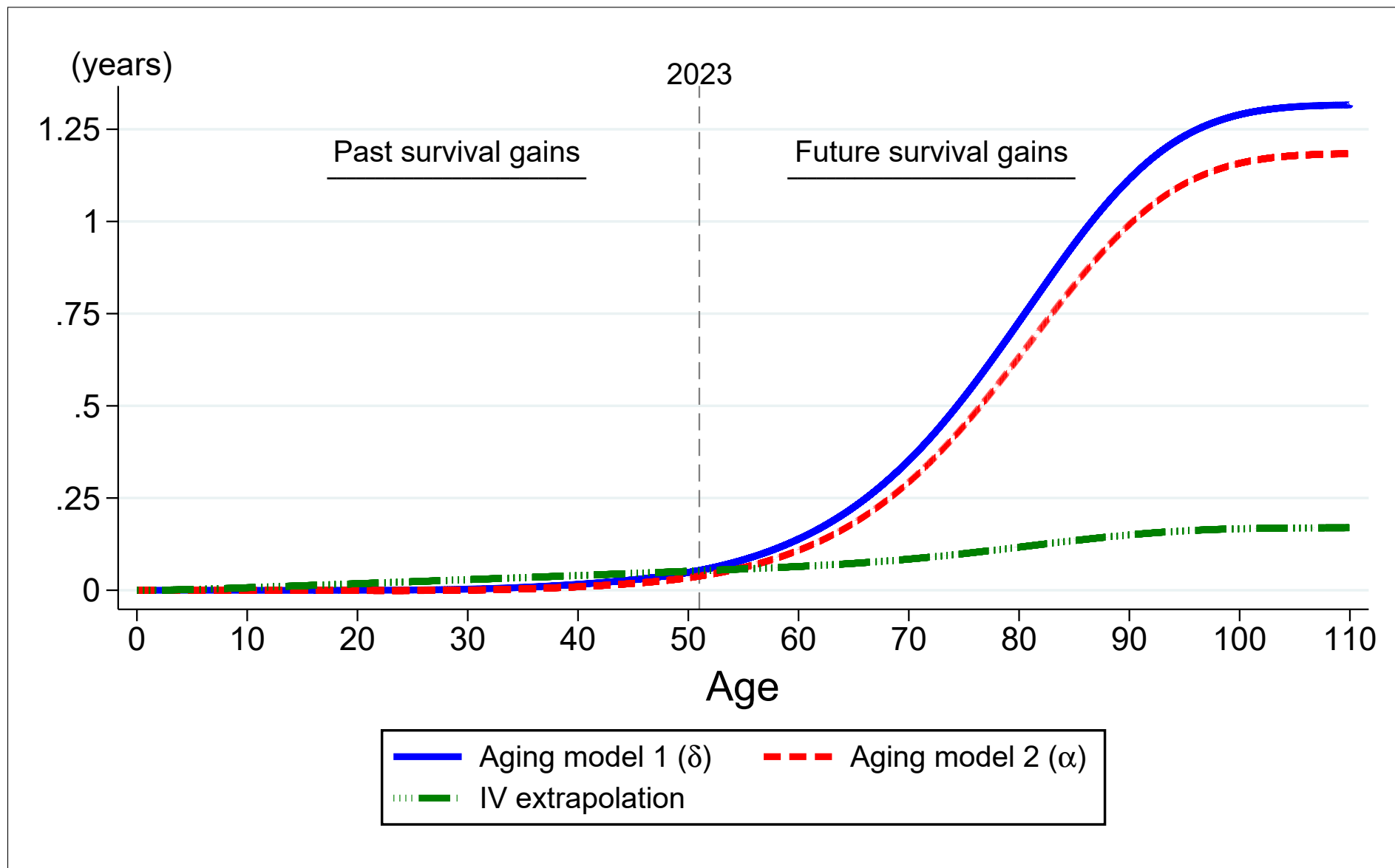
Figure VII: Projected effect of a permanent 1-unit decrease in SO 2 on survival gains for cohort born in 1972
