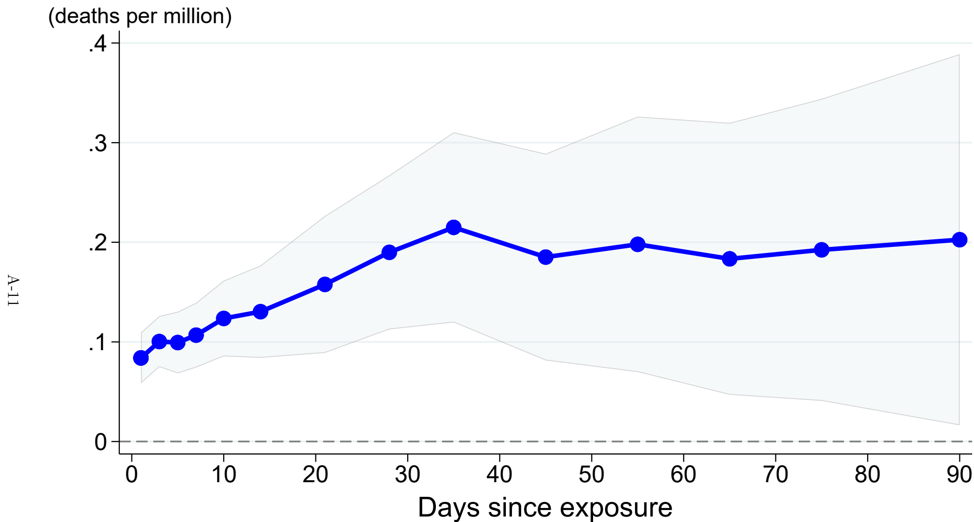
Figure A.7: IV estimates of effect of acute (1-day) SO 2 exposure on cumulative mortality up to 90 days following exposure
