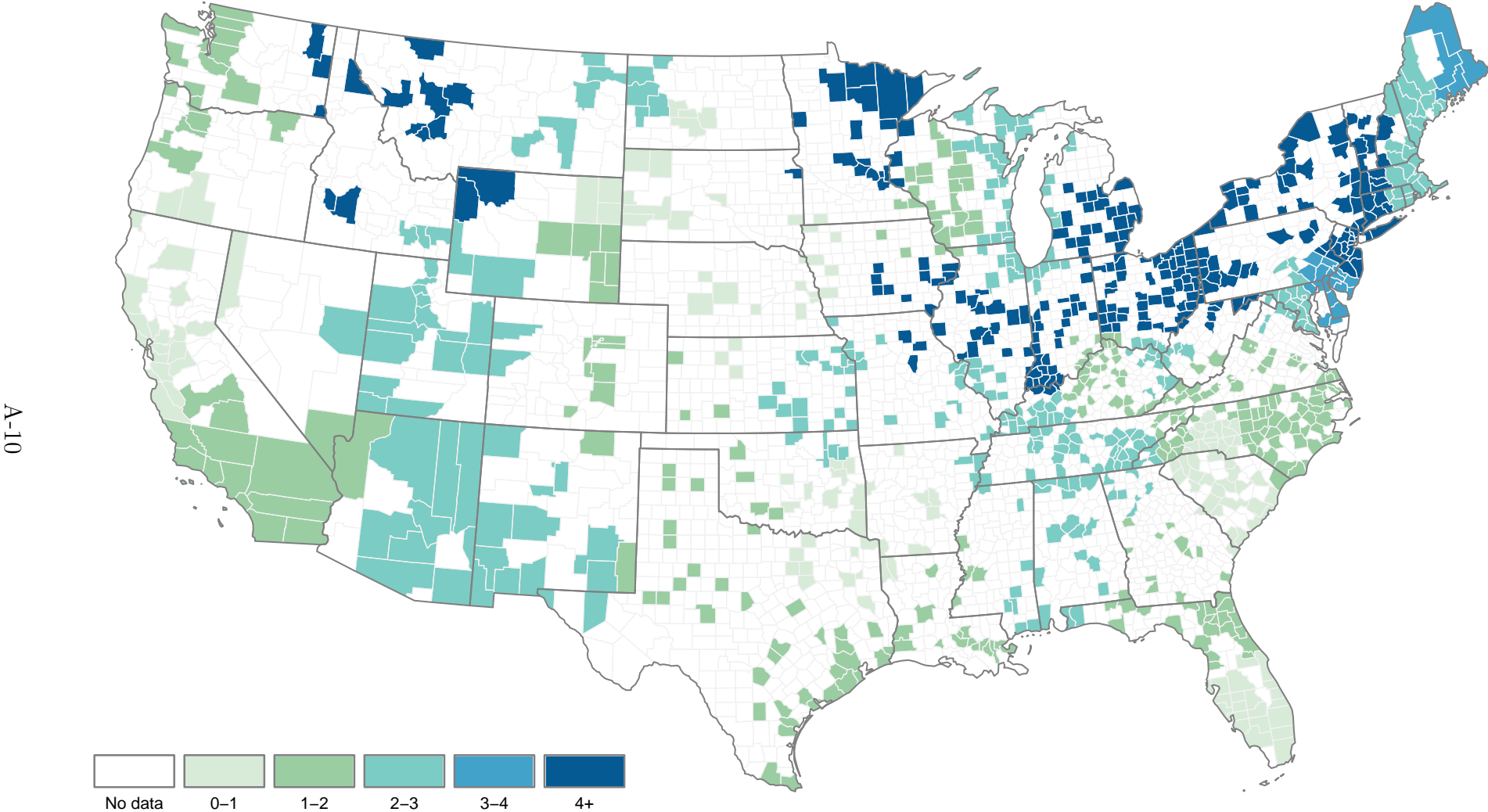
Figure A.6: Strength of the first stage, by geographic group
