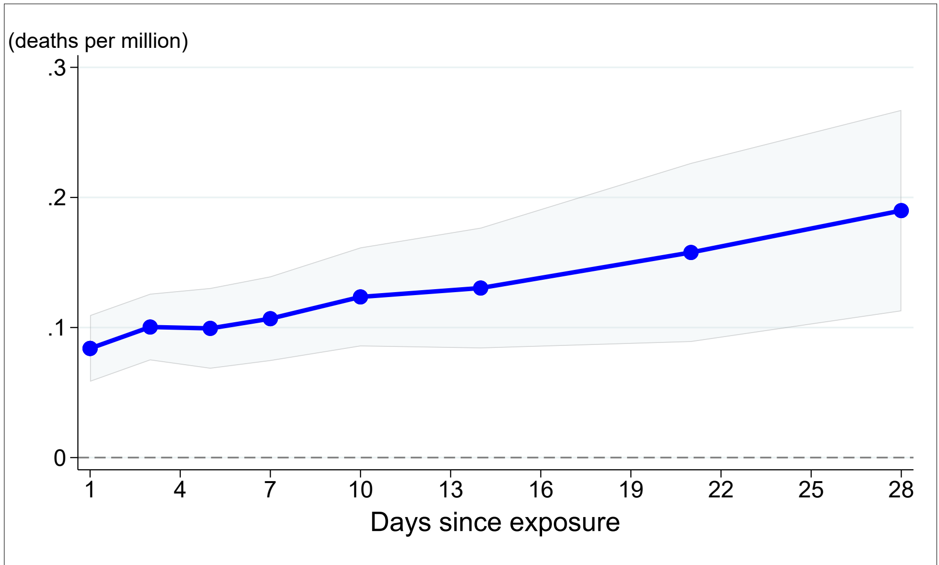
Figure II: IV estimates of effect of acute (1-day) SO 2 exposure on cumulative mortality
