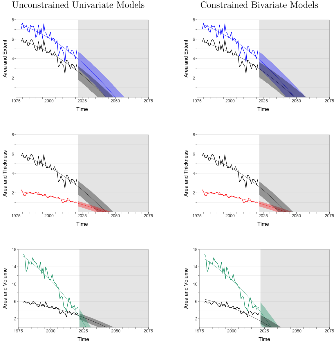
Figure 6: September Arctic Sea-Ice Indicators: Estimated Linear Carbon Trends in Ice-Time Space Under SSP3 7.0 CO 2 Measured as Cumulative Emissions
