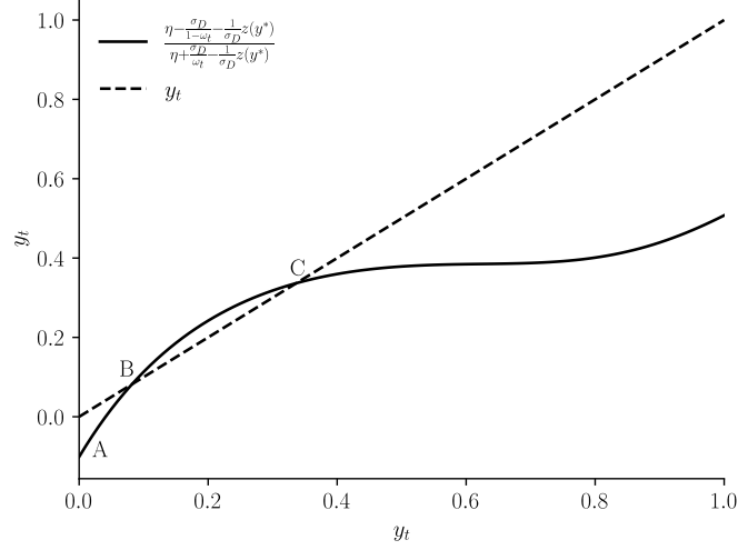
Figure 13: An illustration of Proposition 7.
