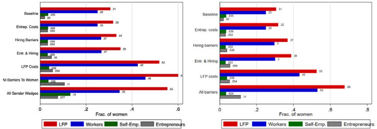
Figure F1: Gender-Specific Ability Distribution and Aggregate Impact
