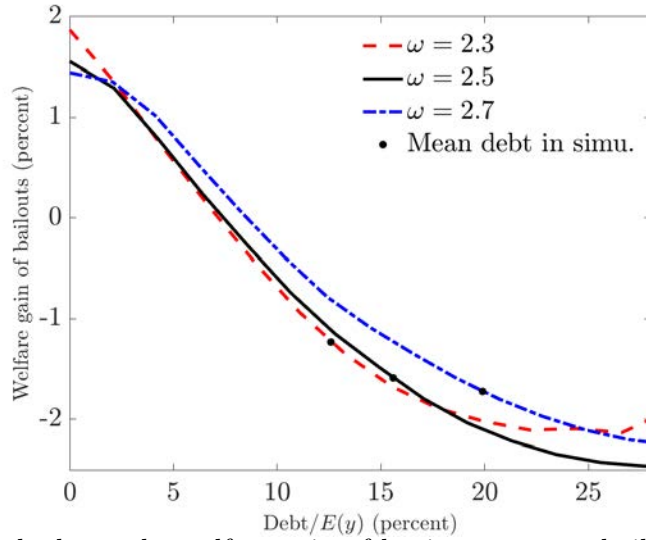
Figure C.2: Welfare gains with different \omega values.
