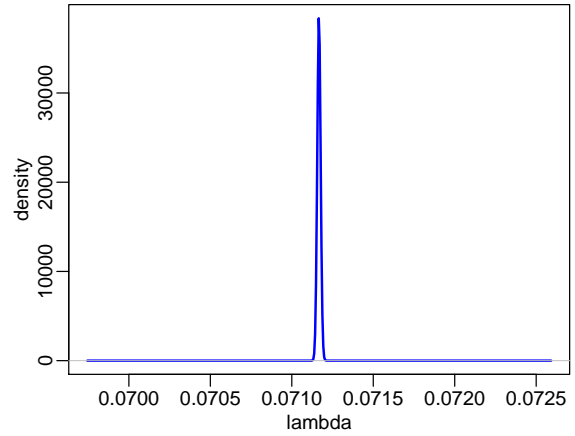
(b) \lambda density of Static Belief model
