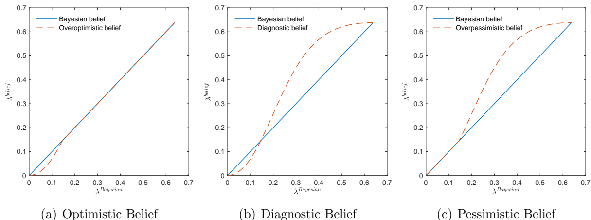
Figure 20: Functional forms of Different Beliefs Derived from Diagnostic Beliefs
