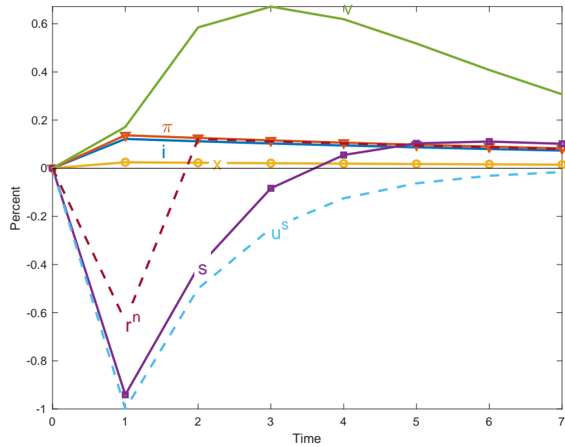
Figure 2: Responses to a fiscal shock with policy rules.
