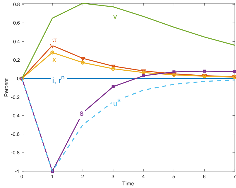
Figure 1: Responses to a fiscal shock with no policy rules.
