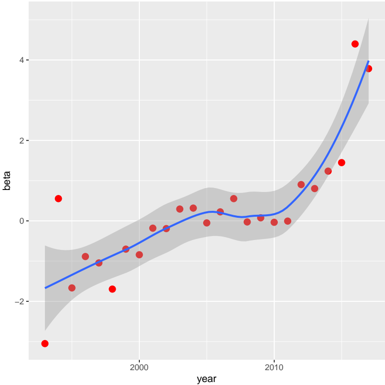
Figure 1: Beta Reputation
