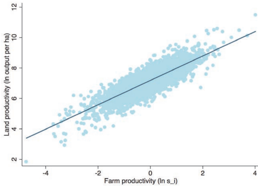
Figure A.3: Yields ( \ln Y/T ) and farm productivity ( \ln s_i )
