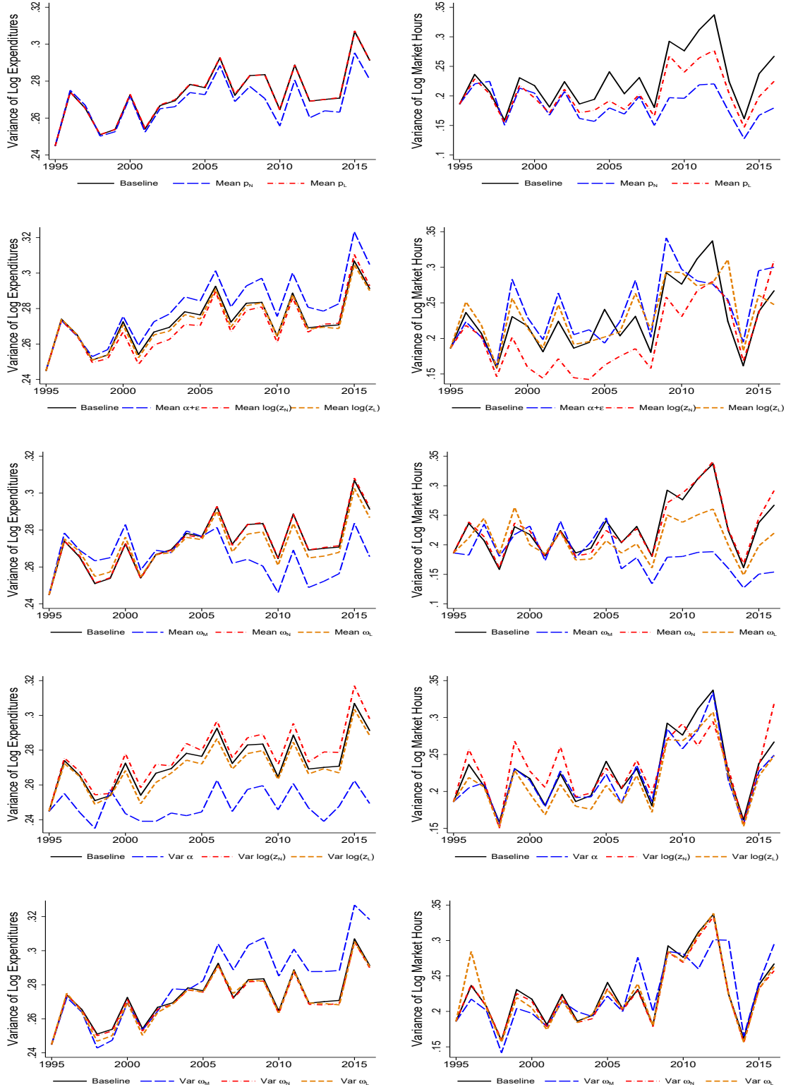
Figure 5: Variances: Counterfactuals
