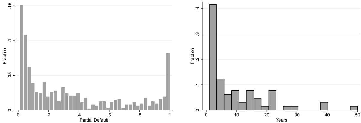
(a) Partial Default Histogram (from panel data) (b) Default Episode Length (from 64 episodes)
