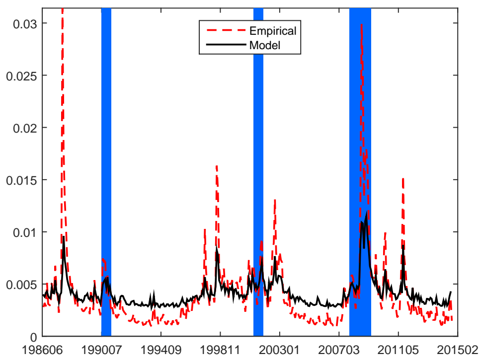
Figure 3: Model-implied and empirical risk-neutral conditional variances of equity market returns. The shaded regions are NBER recession months from the NBER website. The two series are 90.06% correlated.
