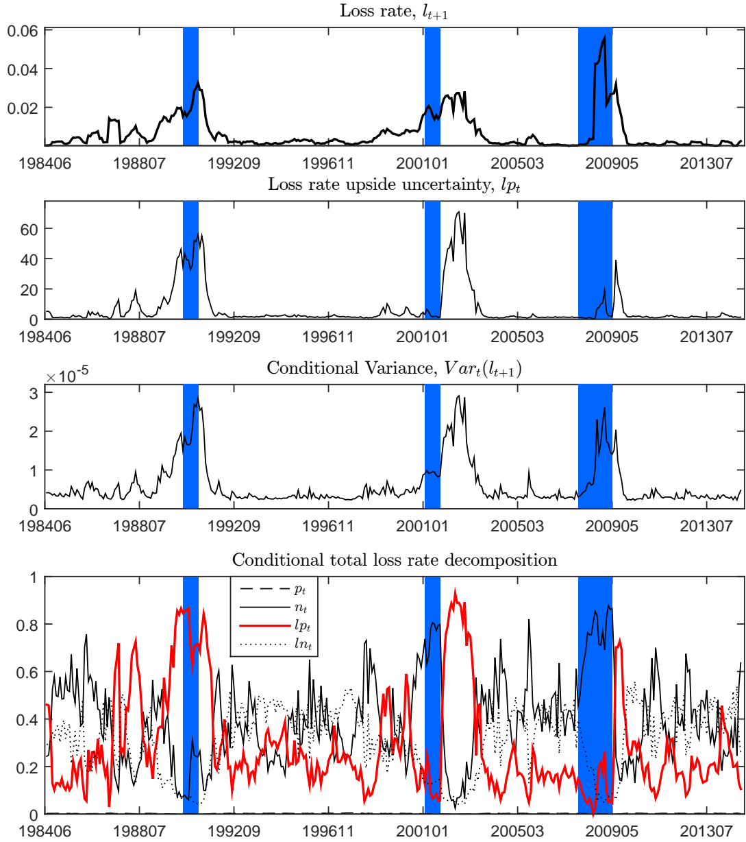
Figure 2: The dynamics and properties of the loss rate. The dynamics and estimation results are shown in Table 2. From top to bottom: loss rate l_{t+1} , the cash flow uncertainty state variable lp_t , the total conditional variance and its decomposition. In particular, there are four independent gamma shocks in the system that contribute to the magnitude and the dynamics of the total loss rate disturbance: real economic shocks, \omega_p and \omega_n , and pure cash flow shocks, \omega_{lp} and \omega_{ln} . The fourth plot depicts the shares of total conditional variances that are explained by each of the shocks at each point of time. Among them, only \omega_{ln} is homoskedastic. The loss rate estimation uses the longest sample available from June 1984 to February 2015. The shaded regions are NBER recession months from the NBER website.
