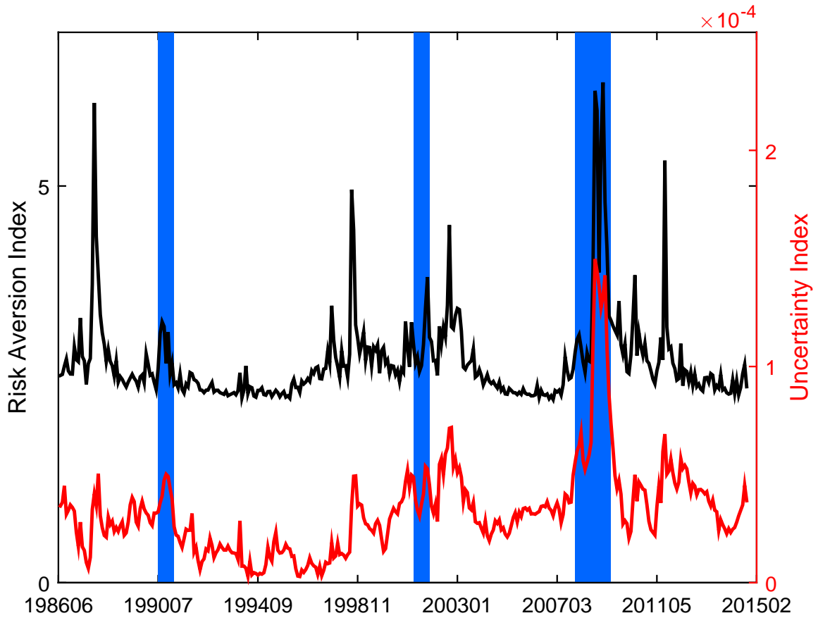
Figure 4: Risk aversion index (black/left y-axis) and Uncertainty index (red/right y-axis). The risk aversion index denoted as ra^{BEX} = \gamma \exp(q_t) and the uncertainty index denoted as unc^{BEX} are linear functions of a set of financial instruments. The utility curvature parameter \gamma is 2. Correlation between the two series is 70.43%. The shaded regions are NBER recession months from the NBER website.
