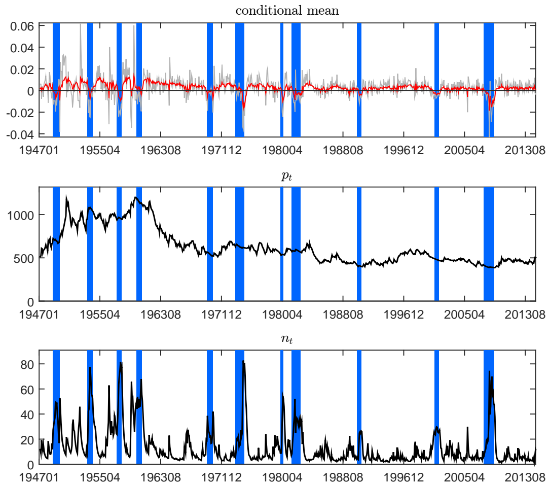
Figure 1: Filtered state variables extracted from industrial production growth. The estimation results are displayed in Table 1. The plot covers the estimation period from January 1947 to February 2015. The shaded regions are NBER recession months from the NBER website.
