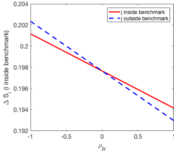
Figure 1: Change in the stockholder value, \Delta S_i , as a function of correlations of project y 's cash flows with cash flows of assets inside and outside the benchmark, \rho_{jy} for some j \leq k and some j > k .
