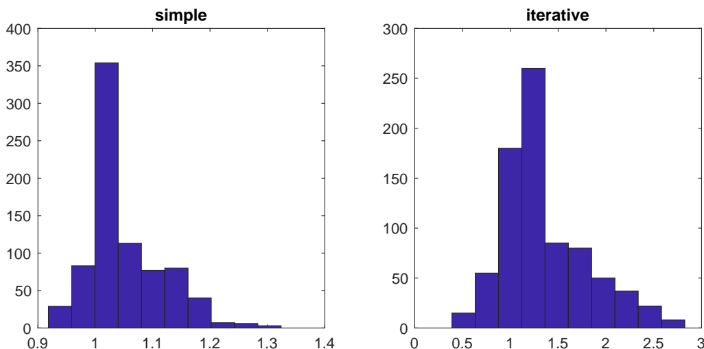
Figure 10: Distribution of \lambda for the US
