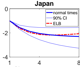
Figure F.1: Impulse response of output to a productivity shock
