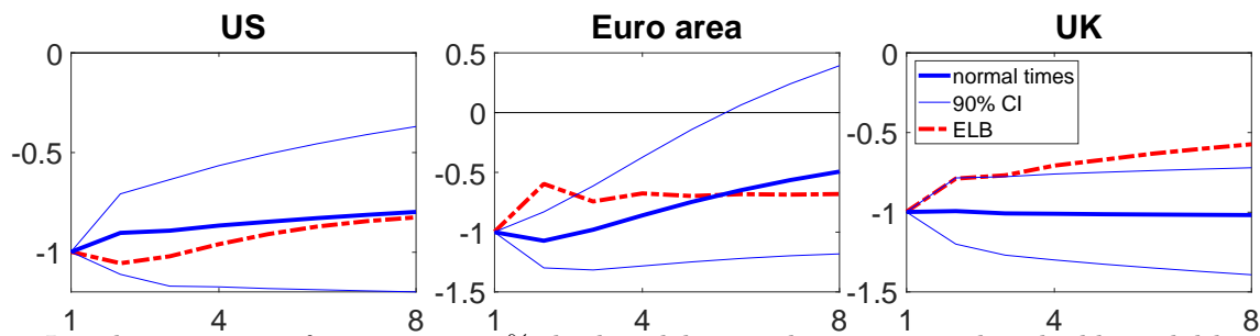
Figure 9: Impulse response of output to a productivity shock
