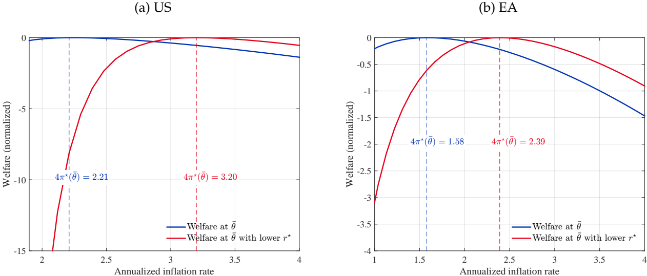
Figure C.1: \mathcal{W}(\pi, \mathbb{E}(\theta))
