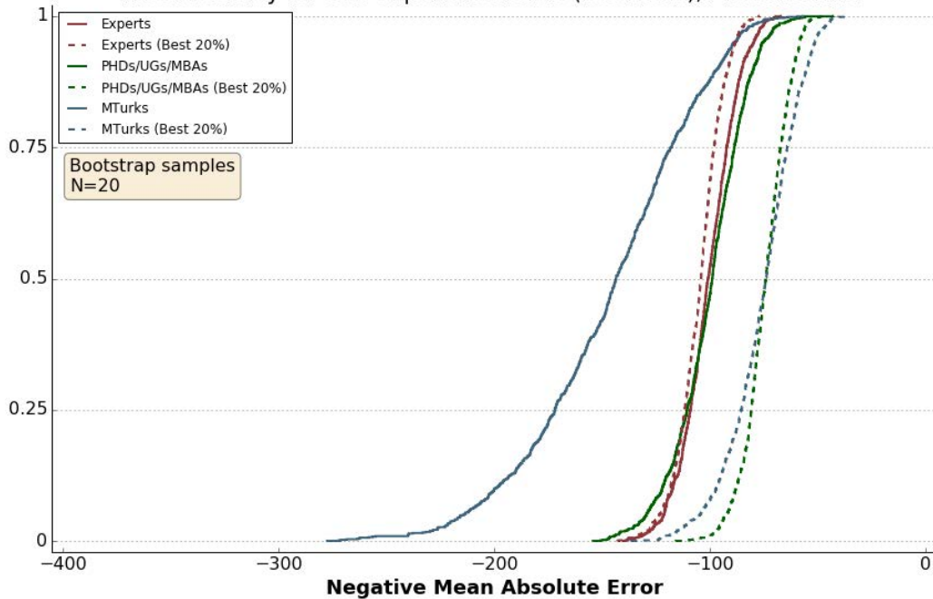
Figure 12b. Wisdom-of-Crowds Accuracy (Groups of 20 Forecasters) WoC Accuracy for OLS Superforecasters (Best 20%), Absolute Error
