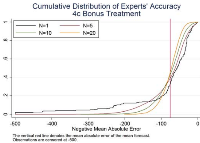
Figure 4. Individual Expert Accuracy versus Aggregate (Wisdom-of-Crowds) Accuracy, Representative Treatments
