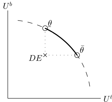
Figure A.5: Pareto frontier
