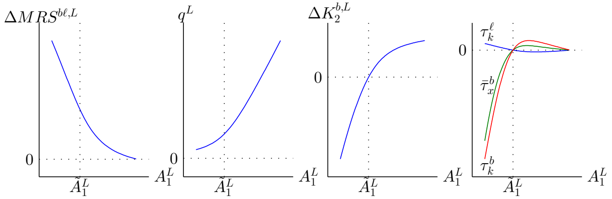
Figure 2: Components of Optimal Taxes \bar{\tau}_x^b , \tau_k^\ell , and \tau_k^b in Application 2
