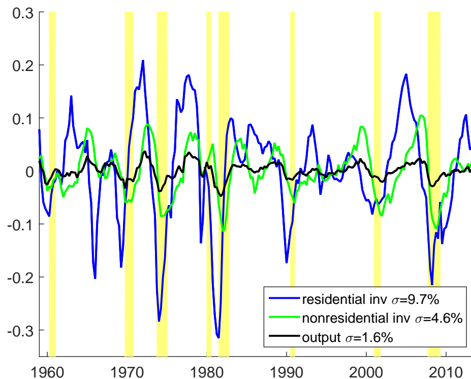
Figure 2: Aggregate residential investment, nonresidential investment and output; logged and detrended with Hodrick-Prescott filter.
