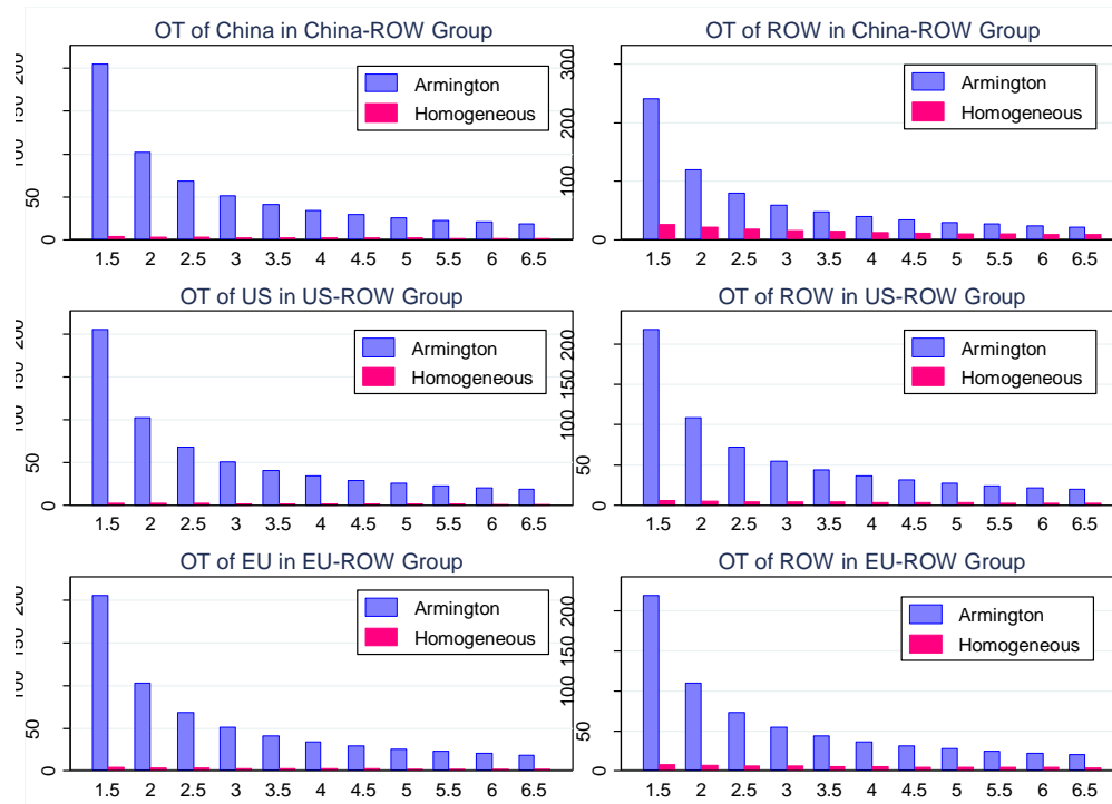
Fig. B2 Sensitivity of Optimal Tariffs to Preference Elasticities under Balanced GE Models
