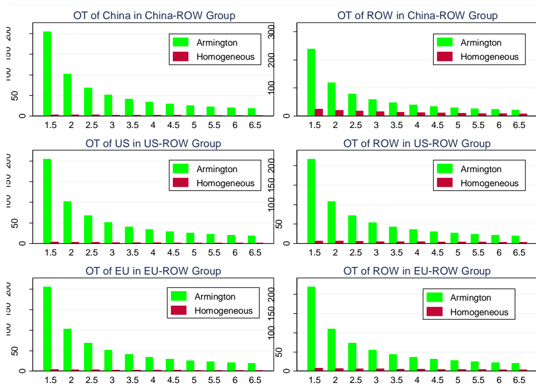
Fig. B3 Sensitivity of Optimal Tariffs to Preference Elasticities under Unbalanced GE Models
