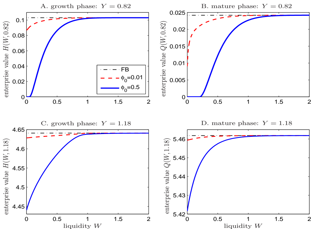
Figure 3: Enterprise values in the growth and mature phases, H(W, Y) and Q(W, Y) . Panels A and B plot H(W, Y) and Q(W, Y) for Y = 0.82 . Panels C and D plot H(W, Y) and Q(W, Y) for Y = 1.18 .
