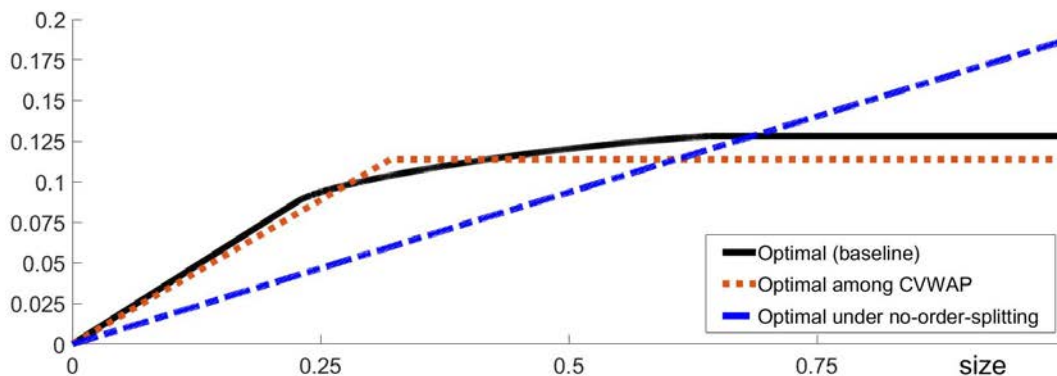
Fig. 5.1: Optimal weighting functions for Example 4
