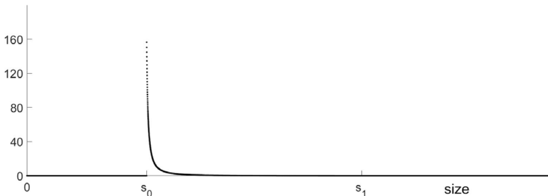
Fig. 4.2: Density of manipulations
