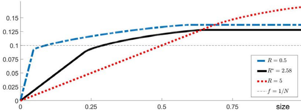
Fig. 4.3: Optimal weighting functions for Example 3
