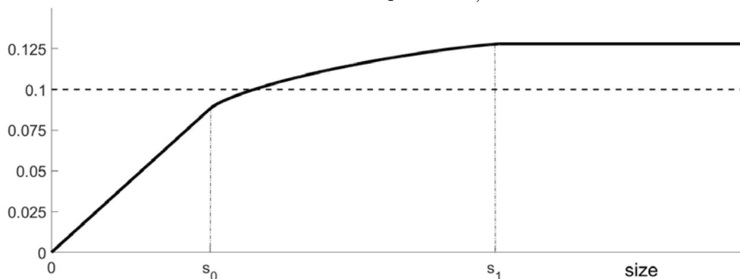
Fig. 4.1: Optimal weighting function for Example 2 (The dotted line depicts the optimal solution in the absence of manipulations)
