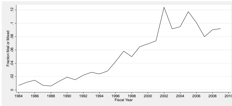
Figure 7: Fraction Mail Ballots, by Fiscal Year
