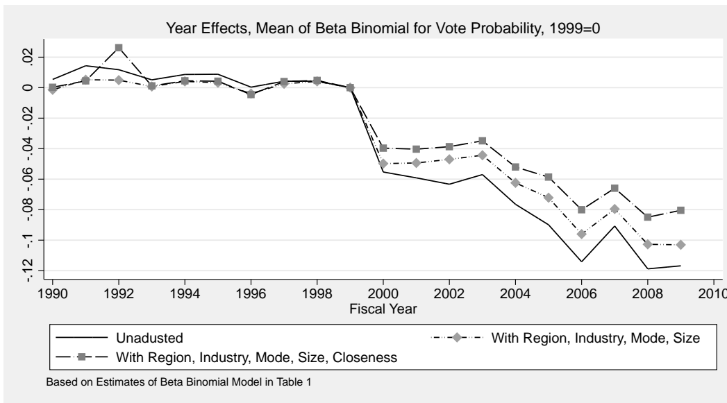
Figure 14: Adjusted and Unadjusted Mean Vote Probabilities, by year.
