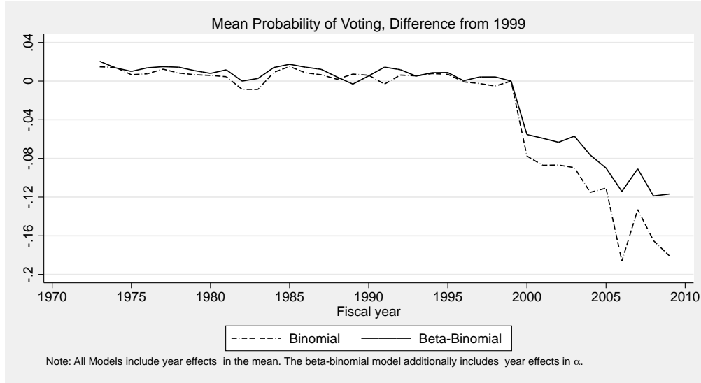
Figure 6: Year Effects in the Mean Probability of Voting (1999=0), 1973-2009.
