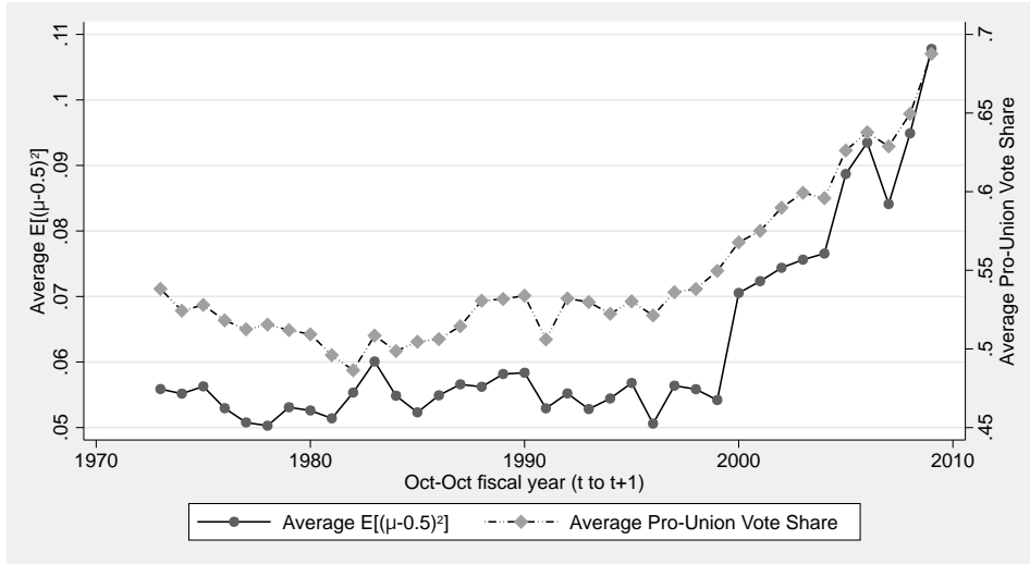
Figure 13: Average Inverse Measure of Closeness ( E((\mu - 0.5)^2|s) ) and Fraction of Vote Pro-Union, by Fiscal Year.
