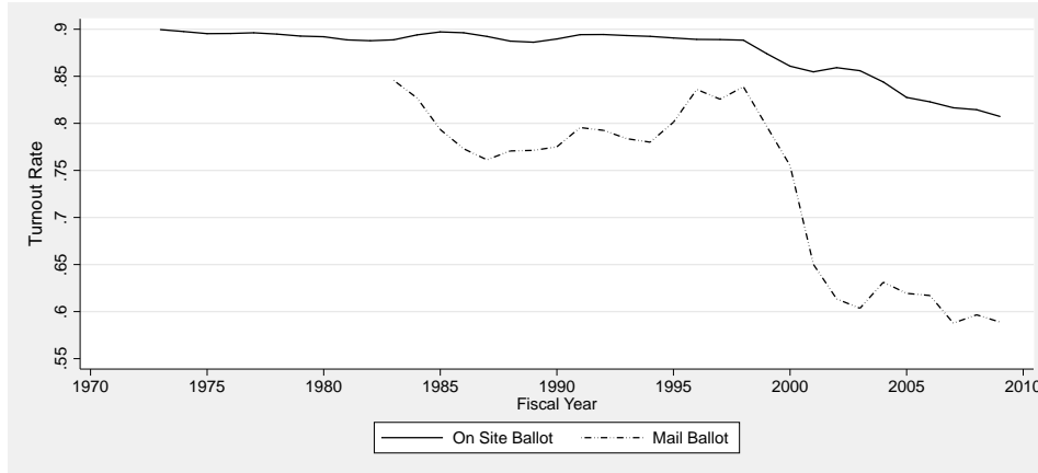
Figure 8: Turnout in On-Site and Mail Elections, by Fiscal Year
