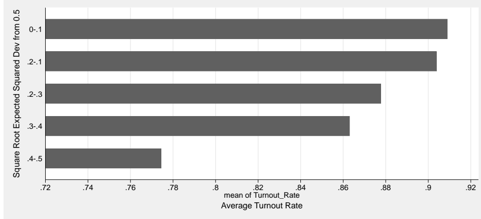
Figure 12: Average Turnout Rate, by Square Root of Expected Squared Deviation of Union Share from 0.5 ( \sqrt{E(\mu - 0.5)^2|s} ).
