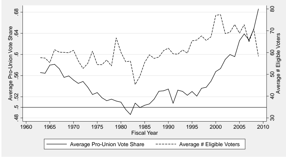
Figure 4: Average Pro-Union Vote Share and Election Size, by Fiscal Year.
