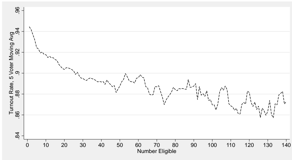
Figure 11: Turnout Rate by Number of Eligible Voters, 5-Voter Moving Average.
