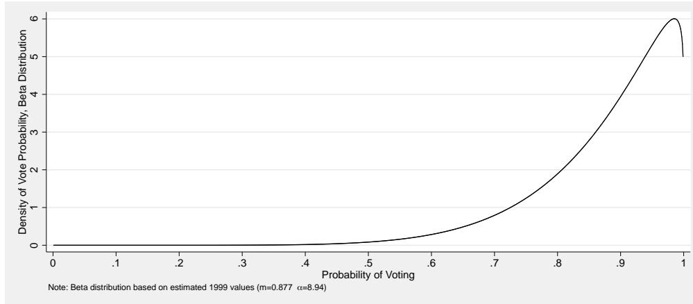
Figure 5: Beta Density Function of Vote Probability (Based on m = 0.877 , \alpha = 8.94 ).
