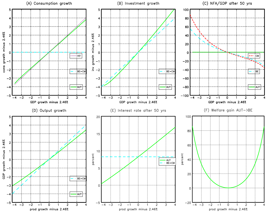
Figure 4: Long-run growth with perfect foresight
