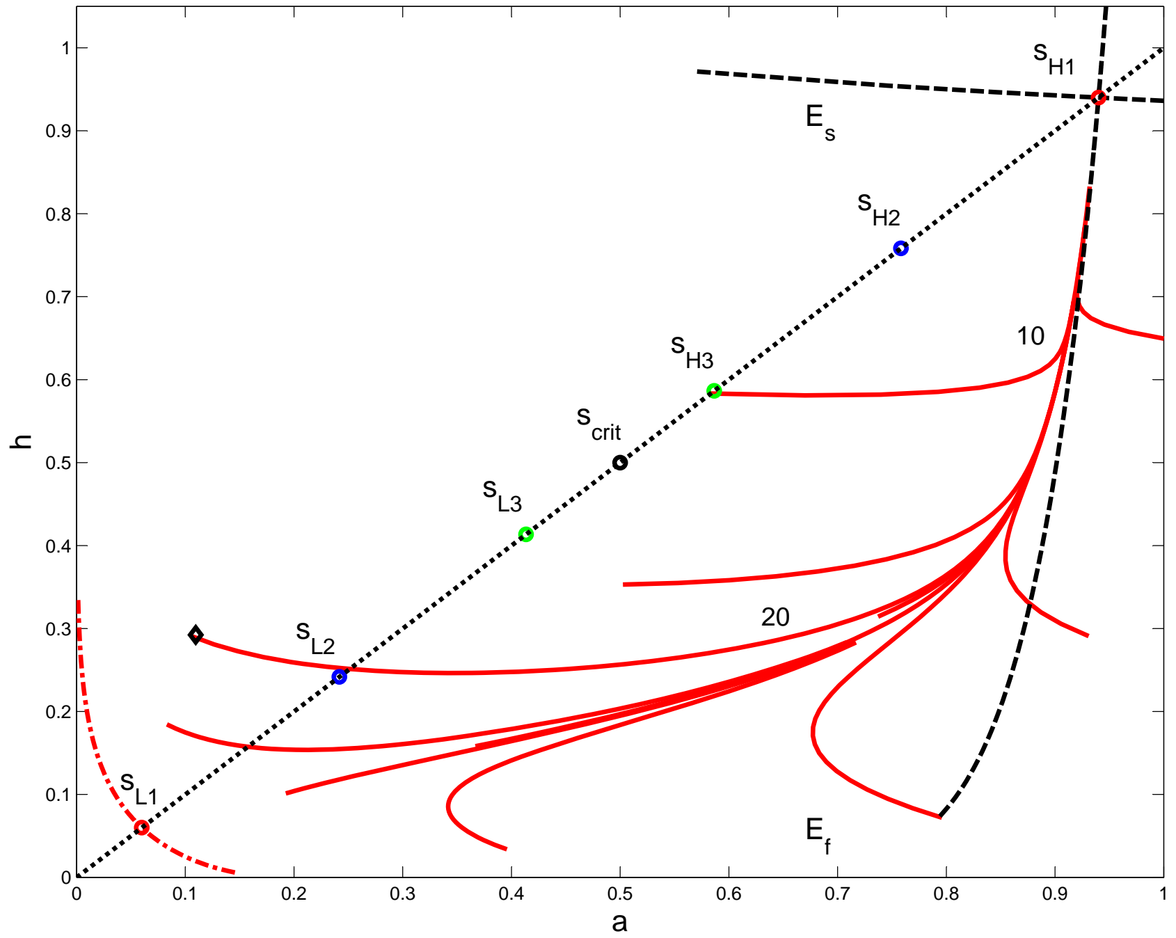
Figure 6: phase diagram, B = 1
