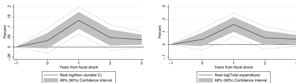
(a) Response of Real Non-dur. Consumption (b) Response of Real Total Consumption
