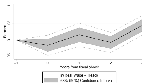
Figure 8: IRFs to a 1% GDP state spending shock: the average response
