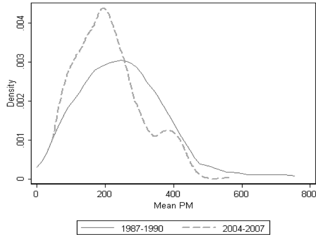
Figure 5A: Kernel Density Graphs of Ambient Air Quality
