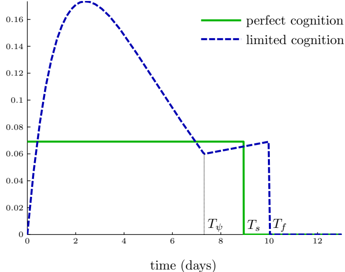
Figure 4: The trading volume under unlimited (green) and limited cognition (blue), when \sigma = 0.3 . In the figure, T_\psi denotes the argument maximum of Q_u .
