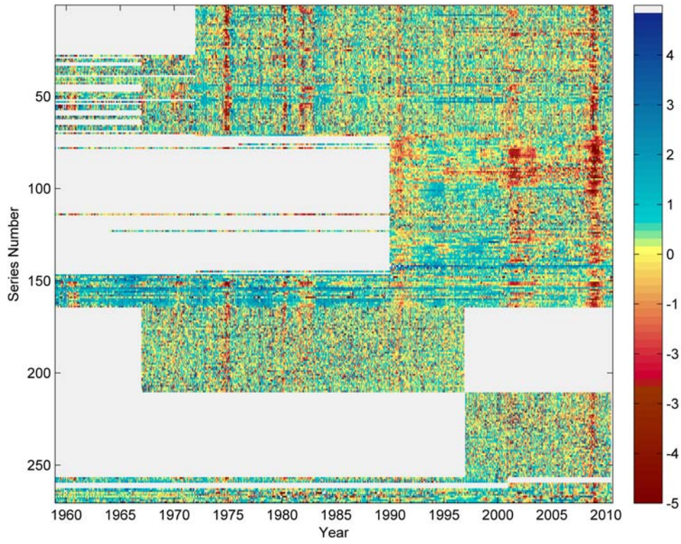
Figure 1. Heat map of monthly growth rates divided by the series standard deviation for the 270 series in the monthly data set. The vertical axis is the series number as given in Appendix A; the horizontal axis is the monthly time scale, 1959:1-2010:9. Negative monthly growth appears as red, positive monthly growth rates appear as blue. The gray sections indicate missing data.
