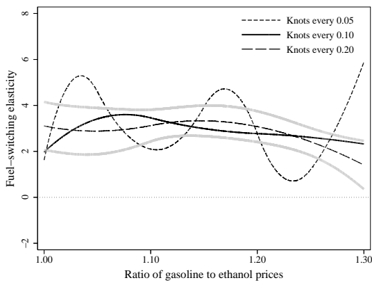
(c) Cubic-spline
