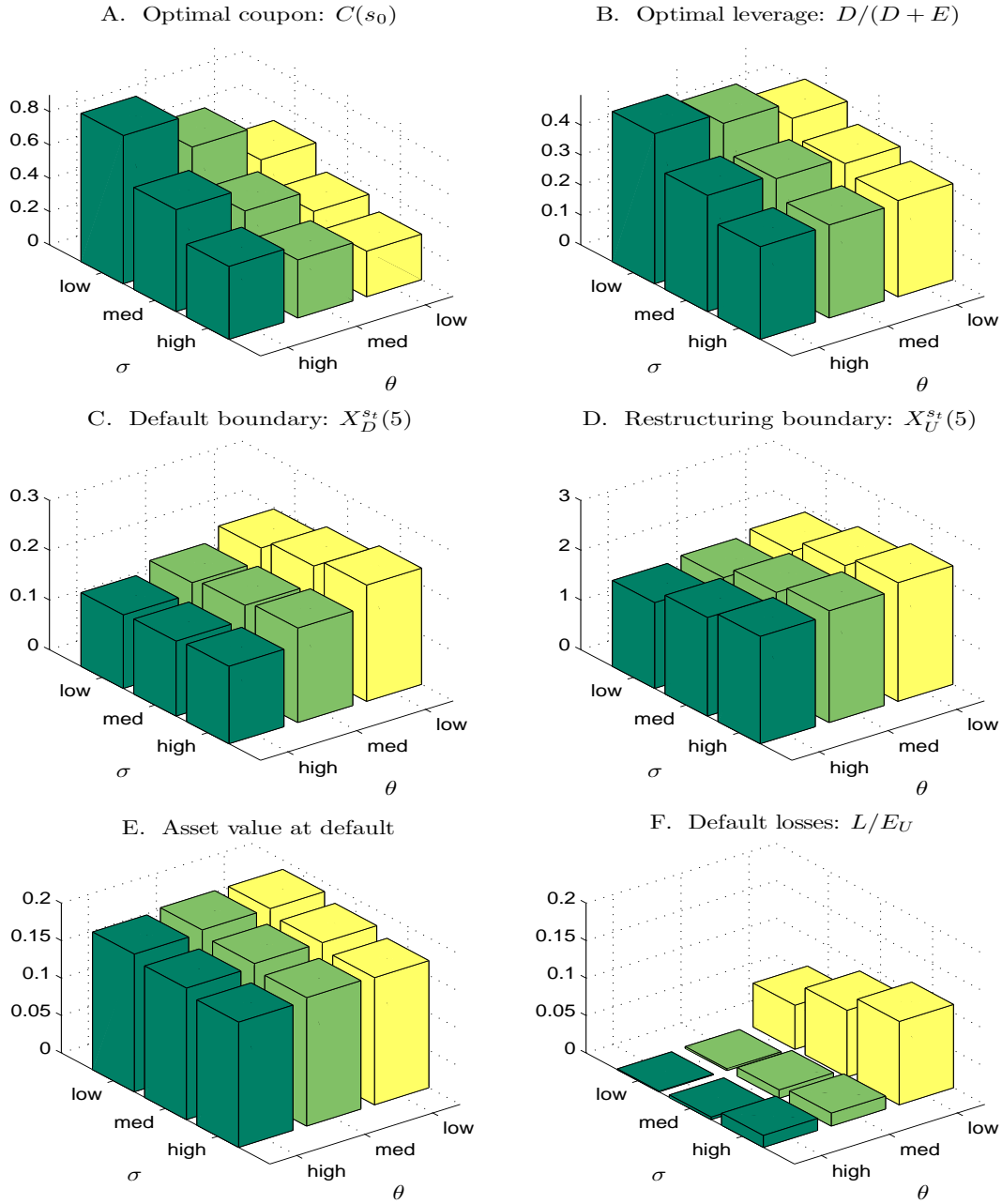
Figure 4. Optimal capital structure, default/restructuring boundaries, asset value at default, and default losses. Panels A and B plot the optimal coupon and leverage ratio the firm chooses in each initial state. Conditional on initial state s_0 = 5 , Panels C through F plot the optimal default and restructuring boundaries, asset value at default (relative to initial asset value), and default losses (relative to initial firm value) in different states. Initial cash flow X_0 = 1 .
