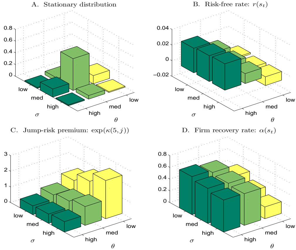
Figure 3. Stationary distribution of the Markov chain, risk-free rate, jump-risk premium, and firm recovery rate. Panel A plots the stationary distribution of the Markov chain. Panels B through D plot the value of the risk-free rate, jump-risk premium, and firm recovery rate in the nine states with different values for the expected growth rate ( \theta ) and conditional volatility ( \sigma ).
