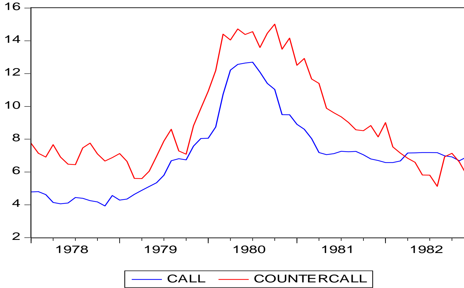
Figure 6-3: Counterfactual 1978-82
