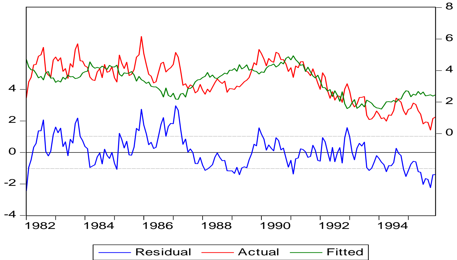
Figure 6-1: Actual value, Fitted value, and residual: call - \pi_{t-1}
