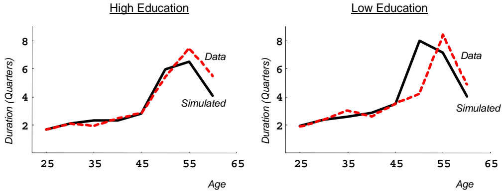
Figure 2: Mean Duration over the Life-Cycle
