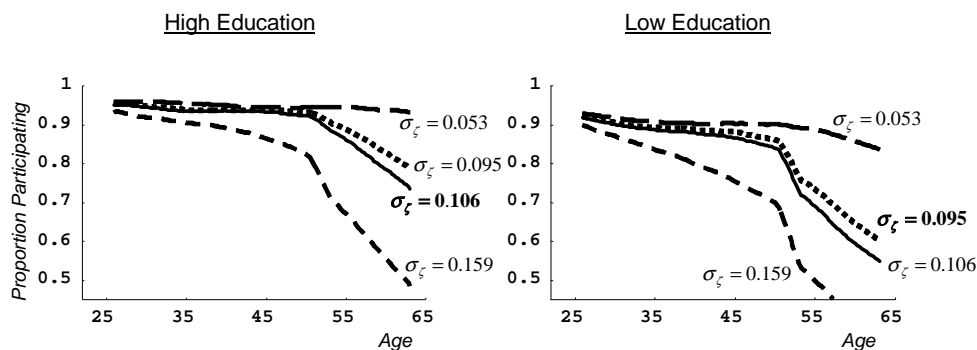
Figure 6: Effect on Employment of Varying \sigma_\zeta
