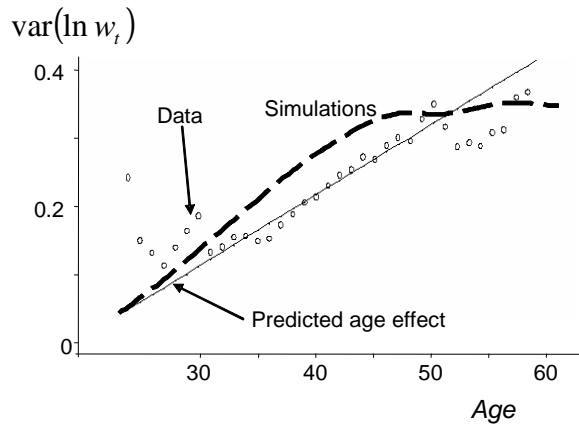
Figure 4: Variance of Wages by Age
