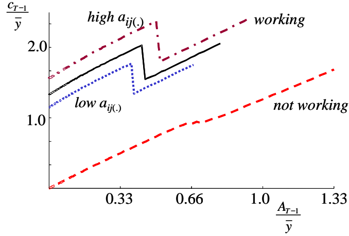
Figure 11: Consumption as a function of current assets conditional on current period work status
