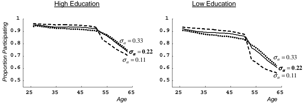
Figure 10: Effect on Employment of Varying Firm Heterogeneity
