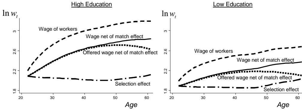
Figure 3: Life-cycle Wage Profiles
