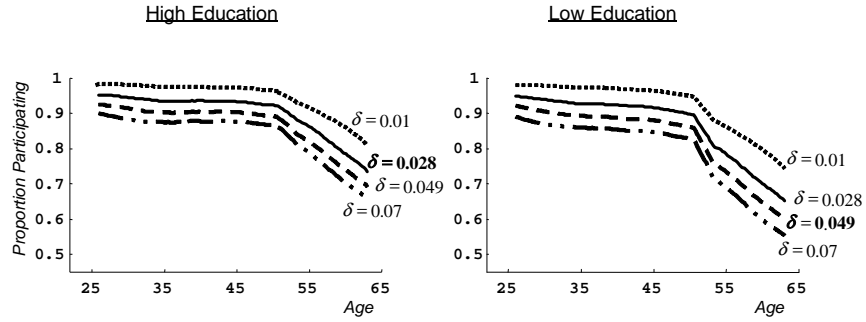
Figure 8: Effect on Employment of Varying Job Destruction
