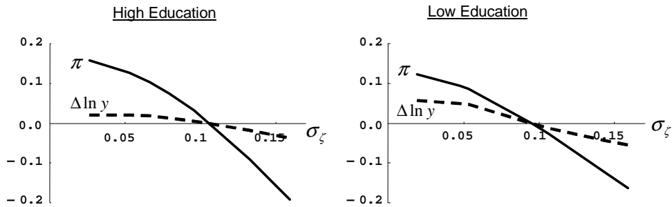
Figure 5: Welfare Costs and Output Effects of Varying \sigma_\zeta
