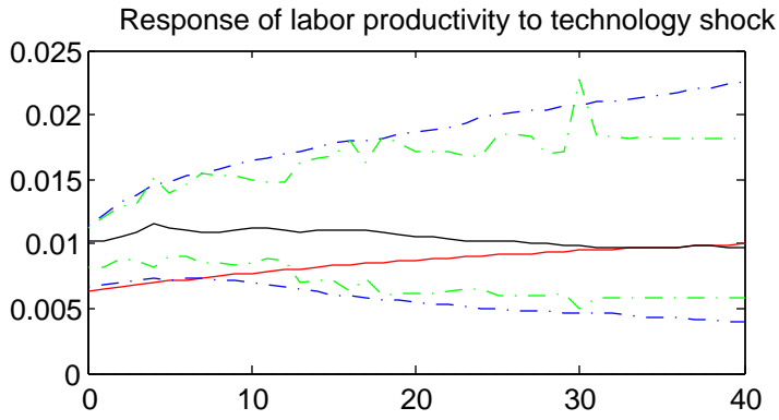
Figure 14: Theoretical and VAR Impulse Responses: Unitary Trade Elasticity
