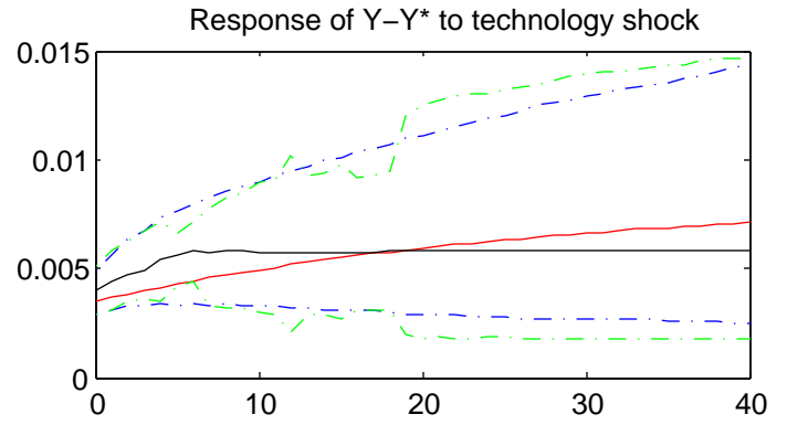
Figure 13: Theoretical and VAR Impulse Responses: High Trade Elasticity
