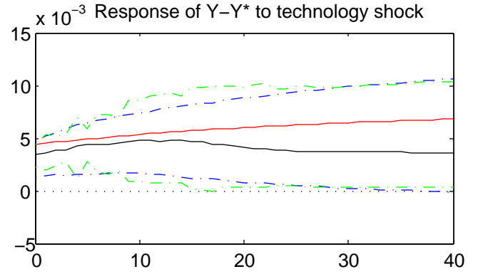
Figure 14: Theoretical and VAR Impulse Responses: Unitary Trade Elasticity
