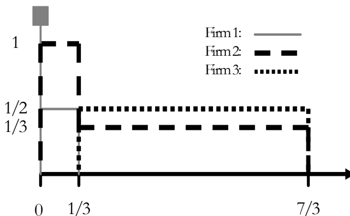
Figure 1: Equilibrium in the Multiplication Game
