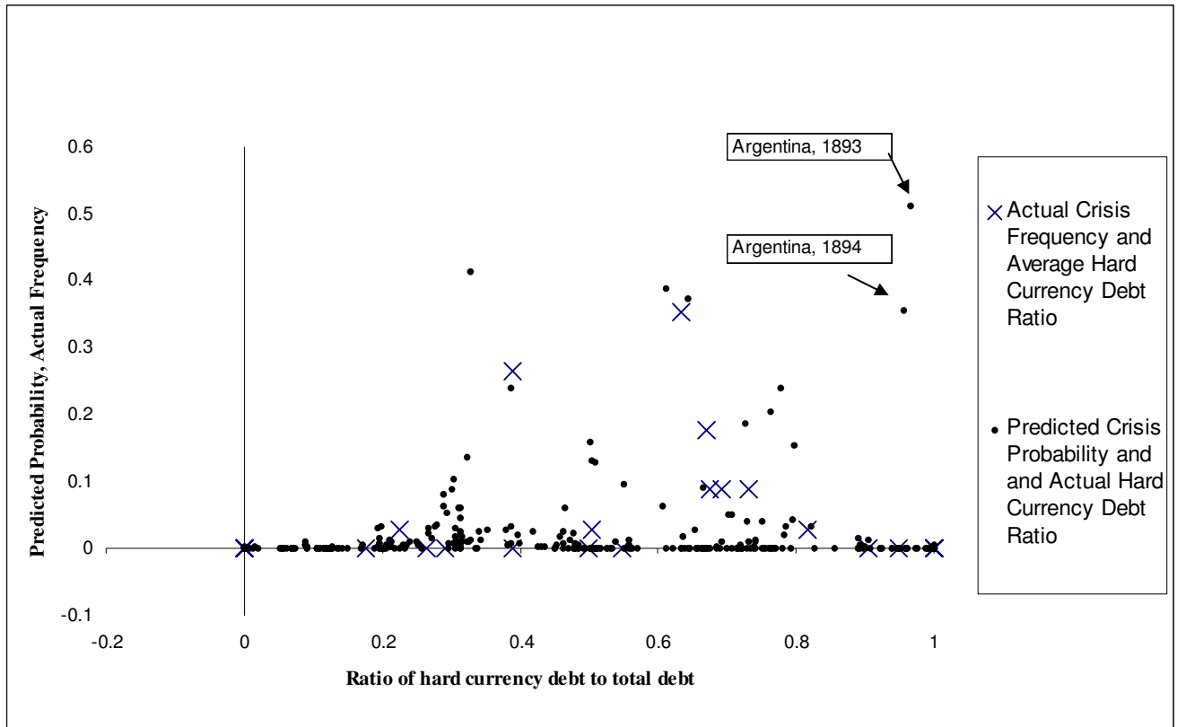
Figure 12 Actual and Predicted Debt Crisis Frequencies by Country versus the Ratio of Average or Actual Hard Currency Public Debt to Total Public Debt, 1880-1913
