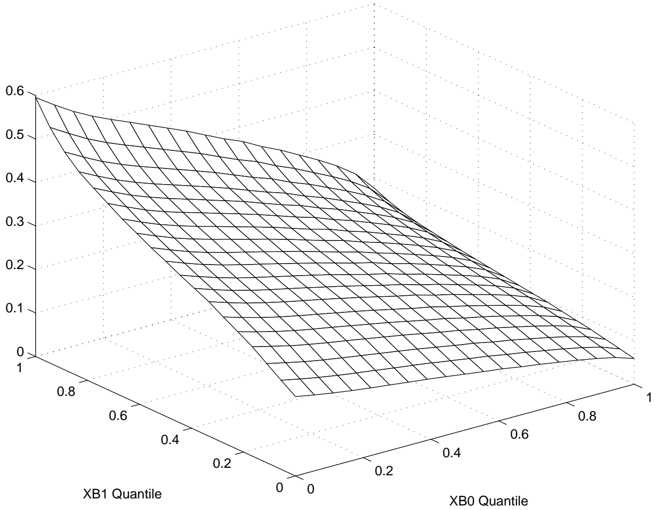
Figure 2: Prob(Delta=1|Xb1, Xb0)
