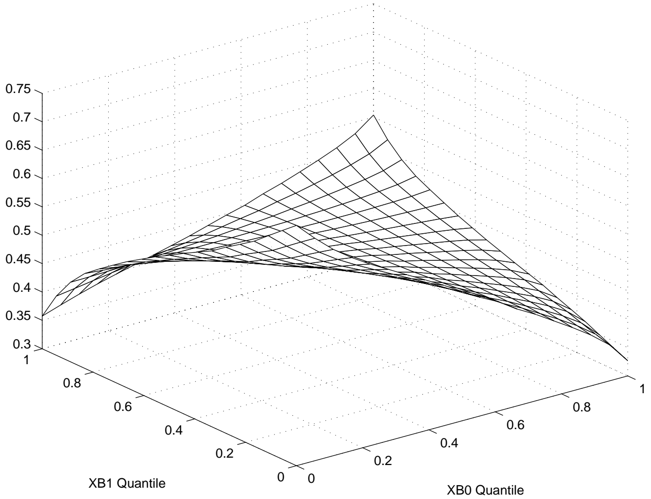
Figure 3: Prob(Delta=0|Xb1, Xb0)
