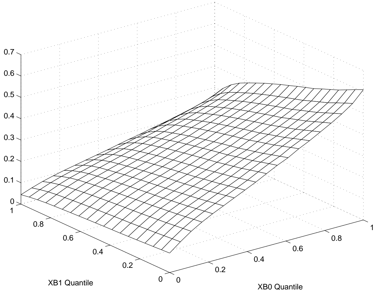
Figure 4: Prob(Delta=-1|Xb1, Xb0)
