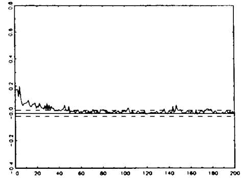
Autocorrelation Function-S&P \epsilon^2 - Jan 41 to Dec 70
