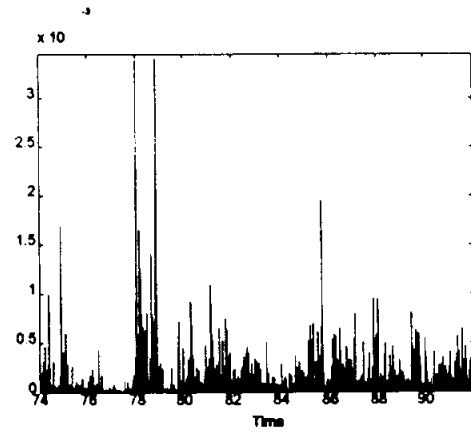
Squared SF/$ Returns (1974-1991)
