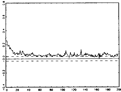
Autocorrelation Function-S&P \epsilon^2 - Jan 28 to Dec 40
