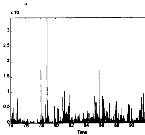
Squared DM/$ Returns (1974-1991)
