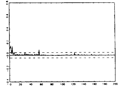
Autocorrelation Function-S&P \epsilon^2 - Jan 81 to May 90
