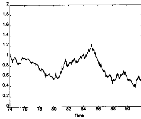
Daily DM/$ Returns (1974-1991)
