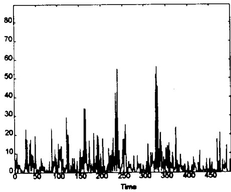
Factor-GARCH Series 1 Squared
