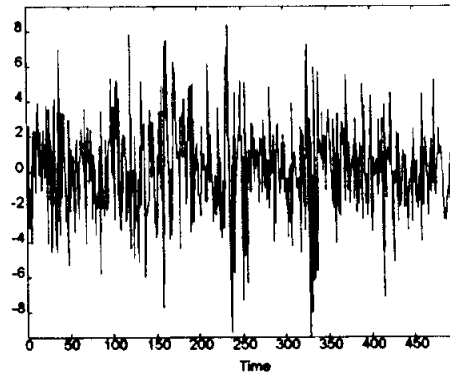
Factor-GARCH Series 2
