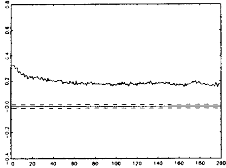
Autocorrelation Function-S&P |\epsilon| - Jan 28 to May 90
