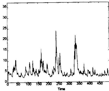
Conditional Covariance
