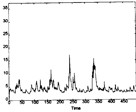
Conditional Variance of Series 1
