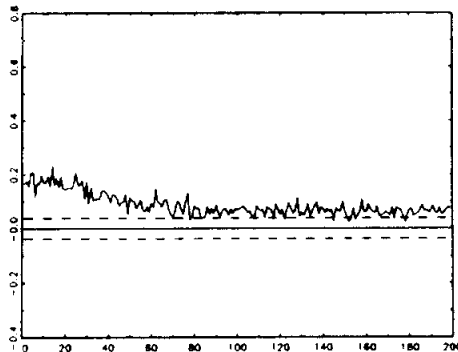
Autocorrelation Function-S&P \epsilon^2 - Jan 71 to Dec 80
