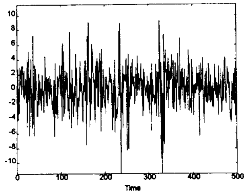
GARCH(1,1) Realization
