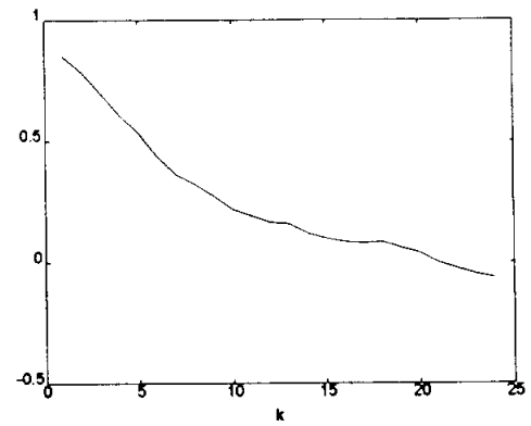
Sample Autocorrelation Function
