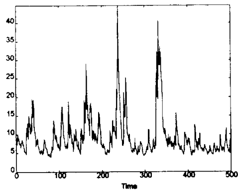
Conditional Variance
