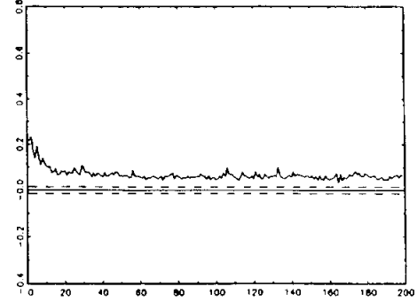
Autocorrelation Function-S&P \epsilon^2 - Jan 28 to May 90
