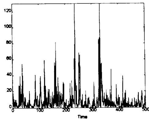
Squared GARCH(1,1) Realization
