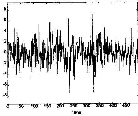
Factor-GARCH Series 1
