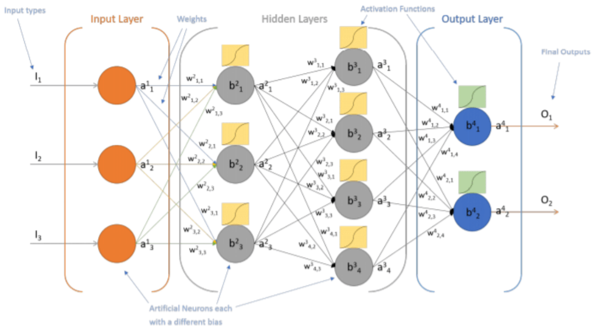
Figure 1. Representation of a Neural Network in LLMs 6
