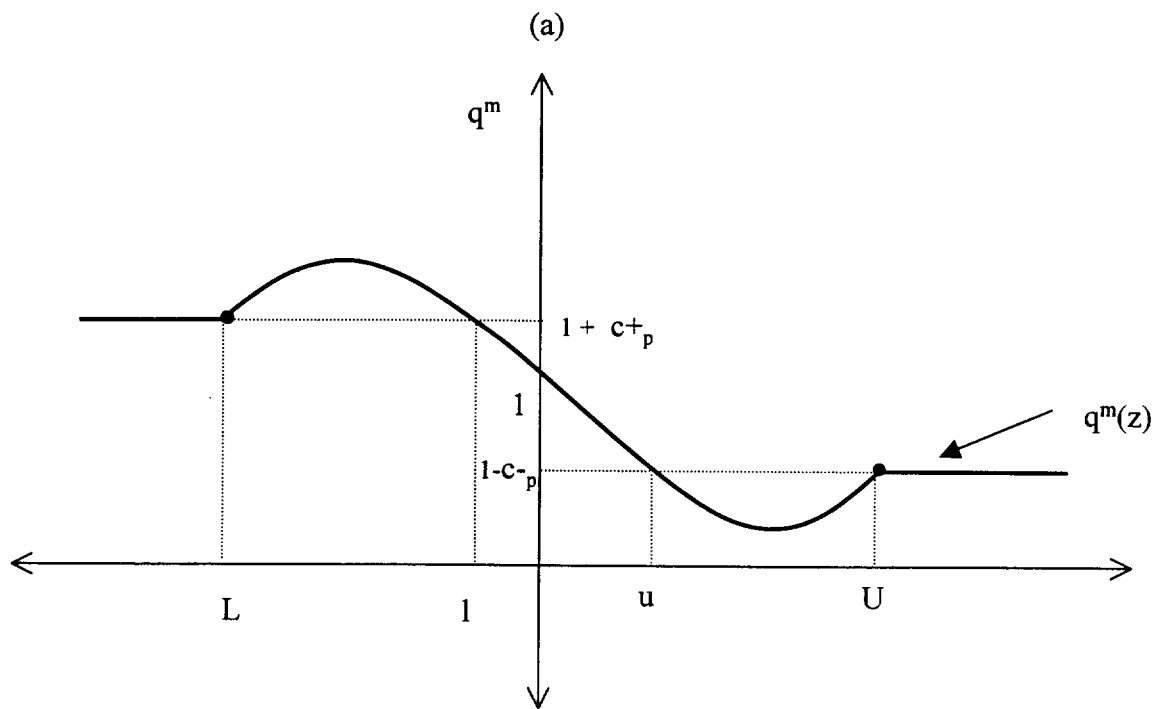
Figure 3.3 Marginal q
