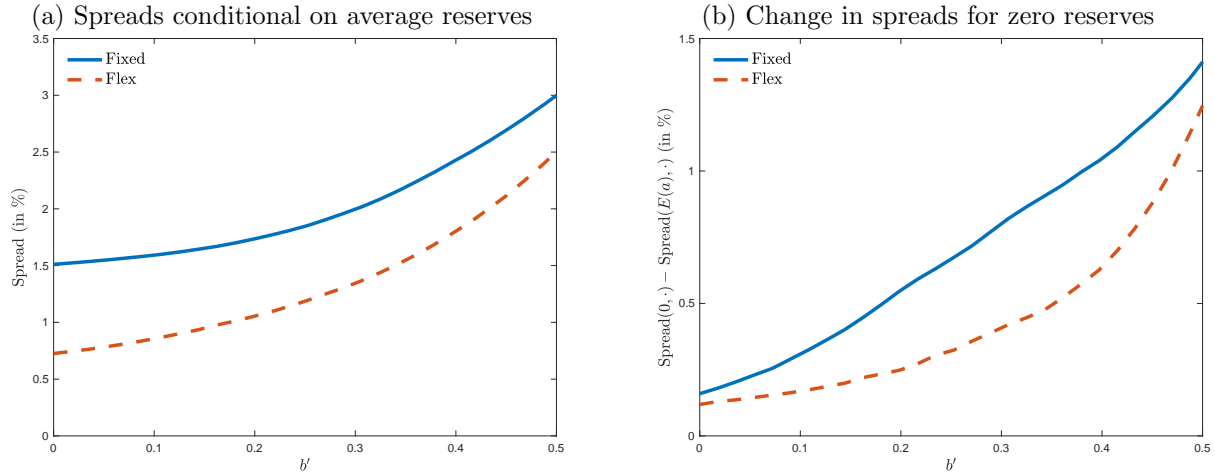
Figure 4: Spread schedules, reserves, and nominal rigidities.
