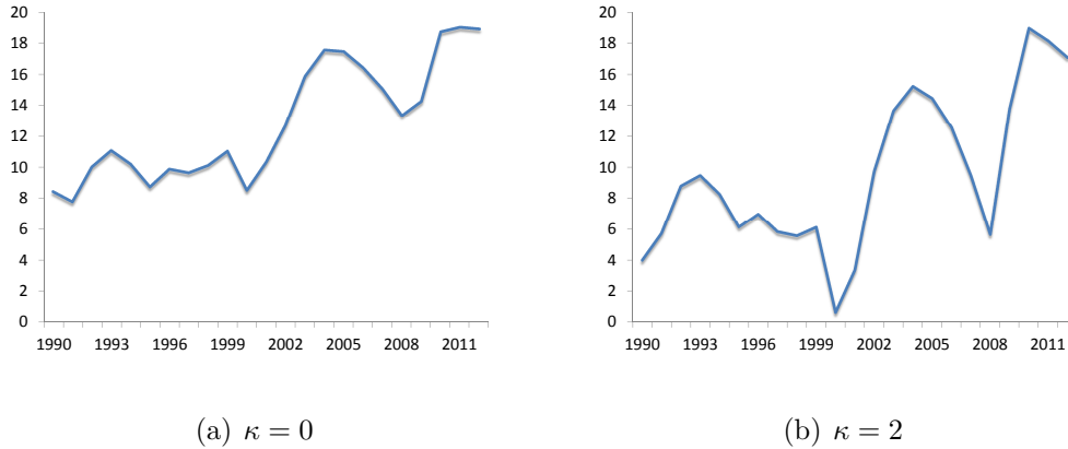
Figure 2: The Capital Wedge for Two Values of the Adjustment Cost \kappa . Source: U.S. NIPAs; see spreadsheets
